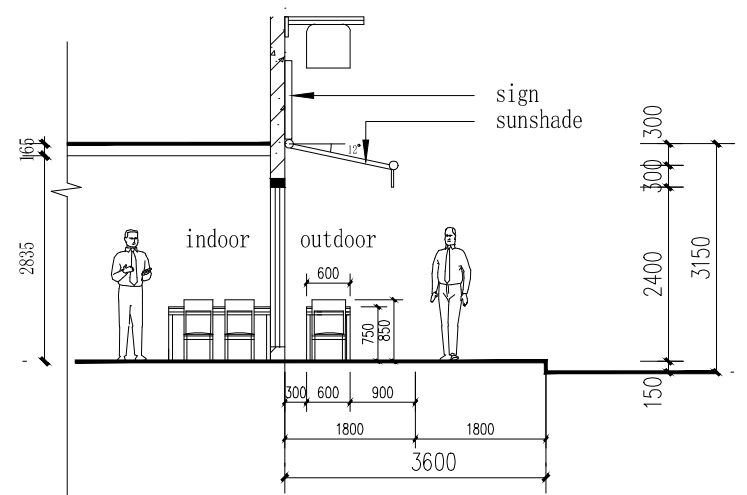
I-I Profile
