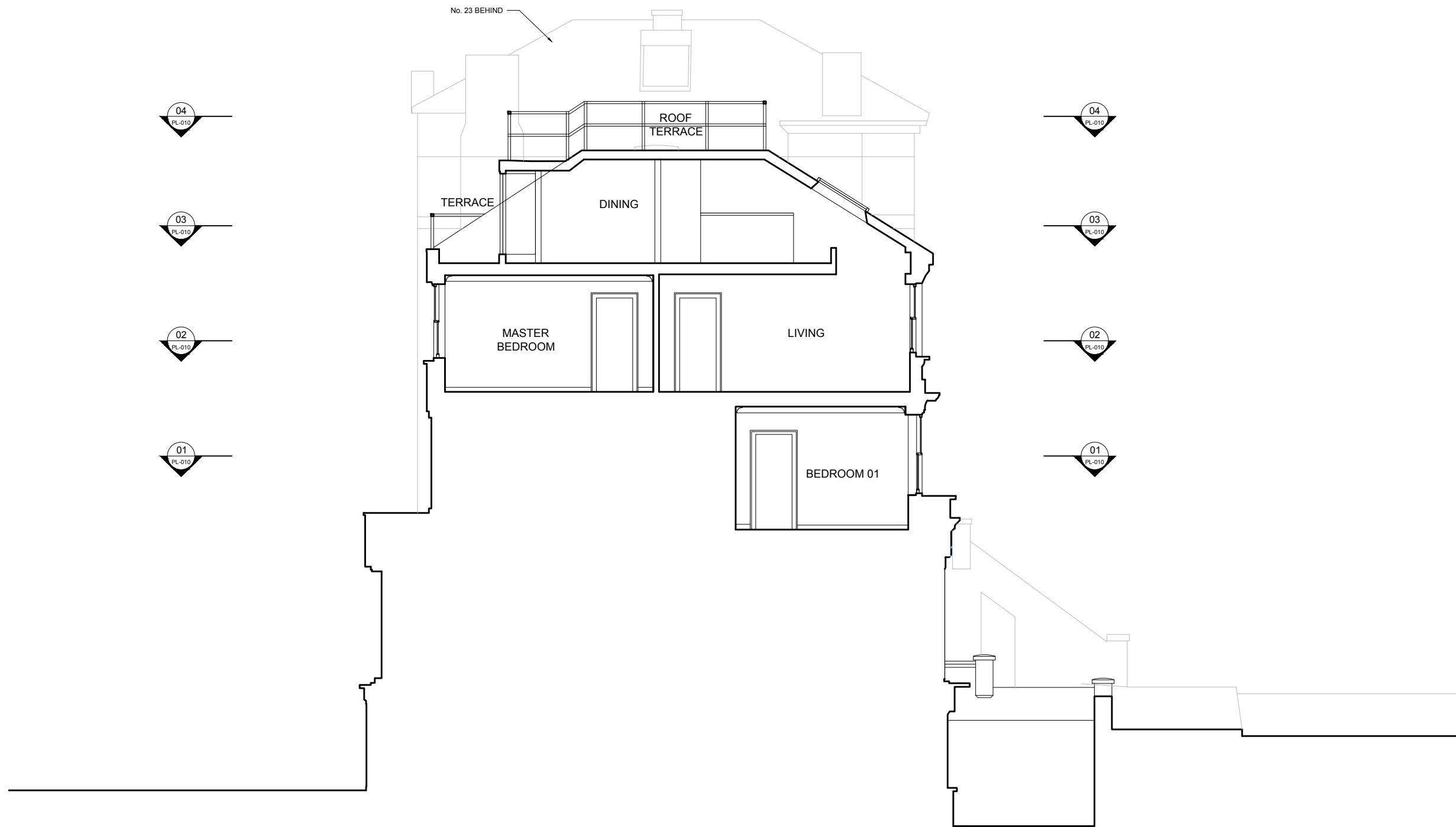
EXISTING SECTION AA SCALE 1:100 @ A3
