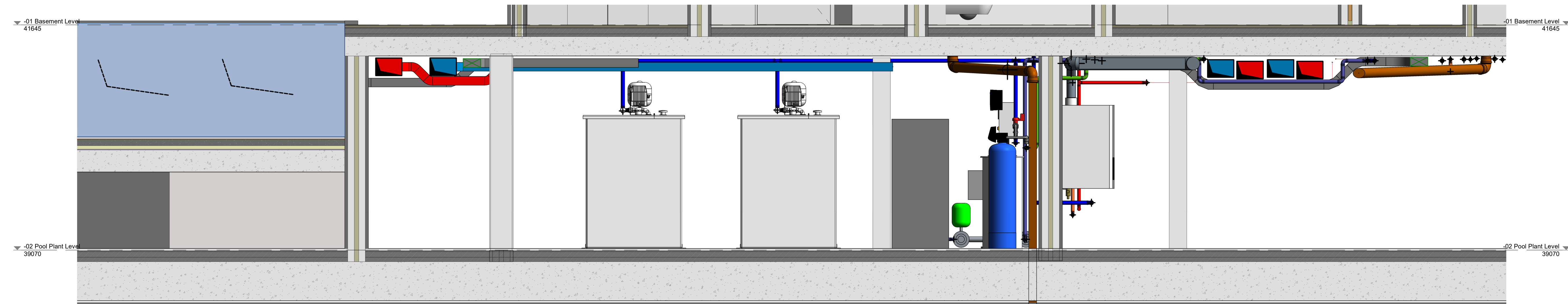
Section C Mechanical Plant Room Section: Cold Water Tank Room
