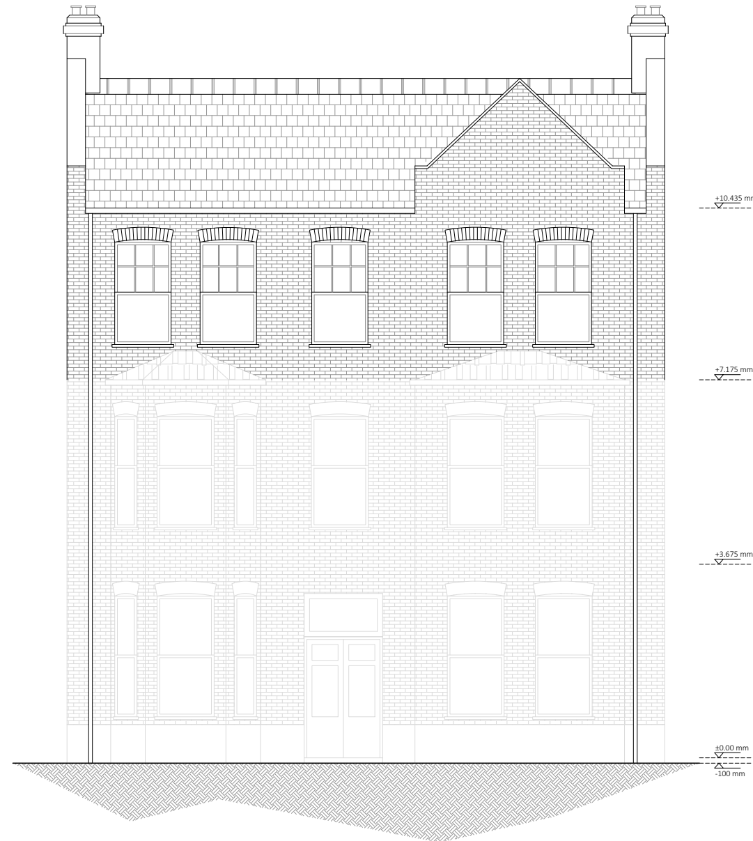
PROPOSED FRONT ELEVATION (NOT CHANGES)
