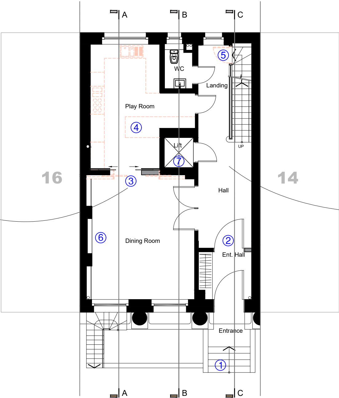
Proposed opening with sliding doors to be as approved / existing at 33 Chester Terrace
