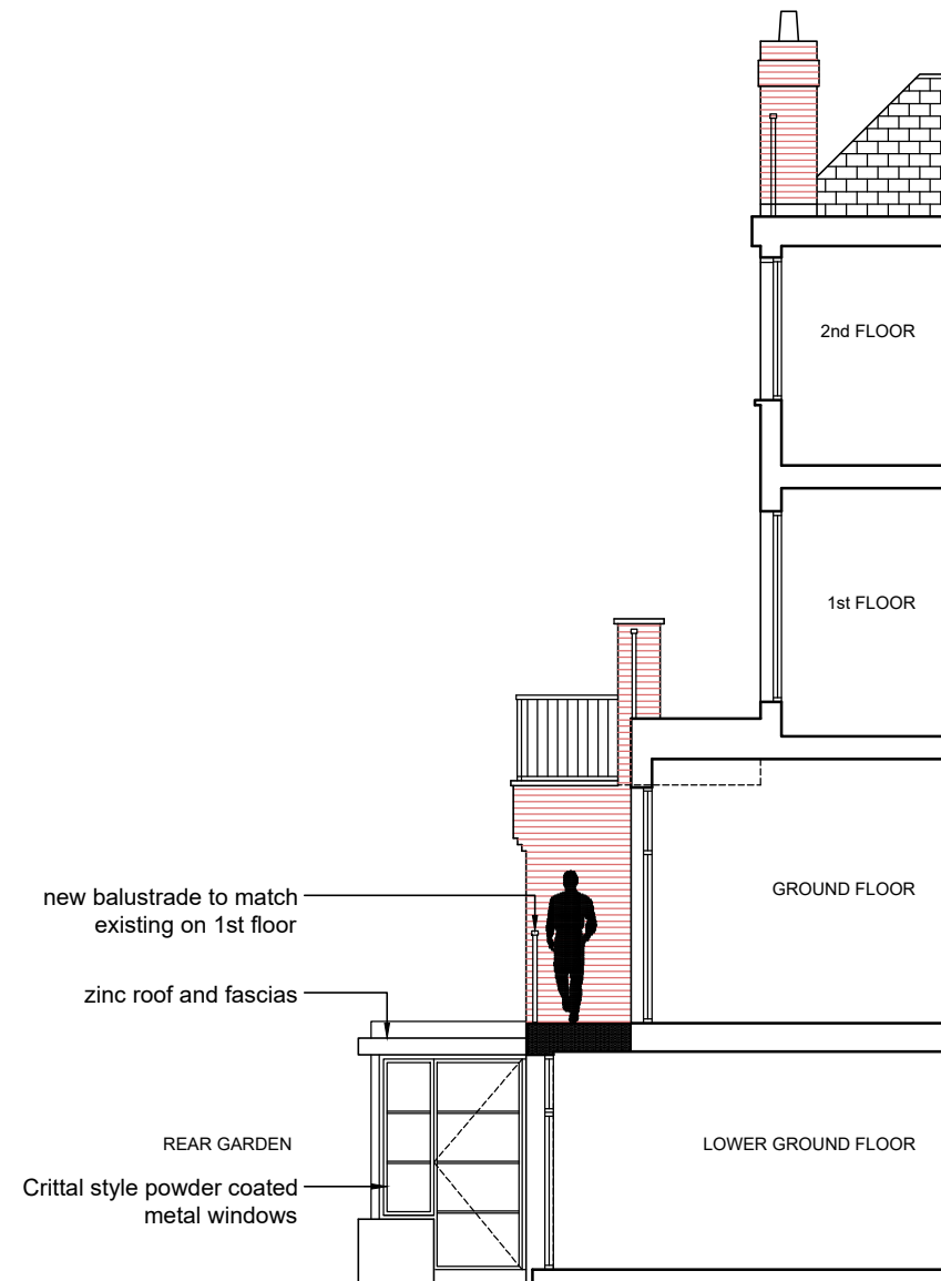
SECTION A
