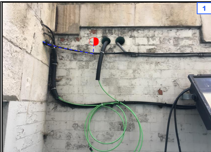
1. Cable to exit via new civils, next to existing colt ducting. 12f cable to run through existing hole into courtyard area.
