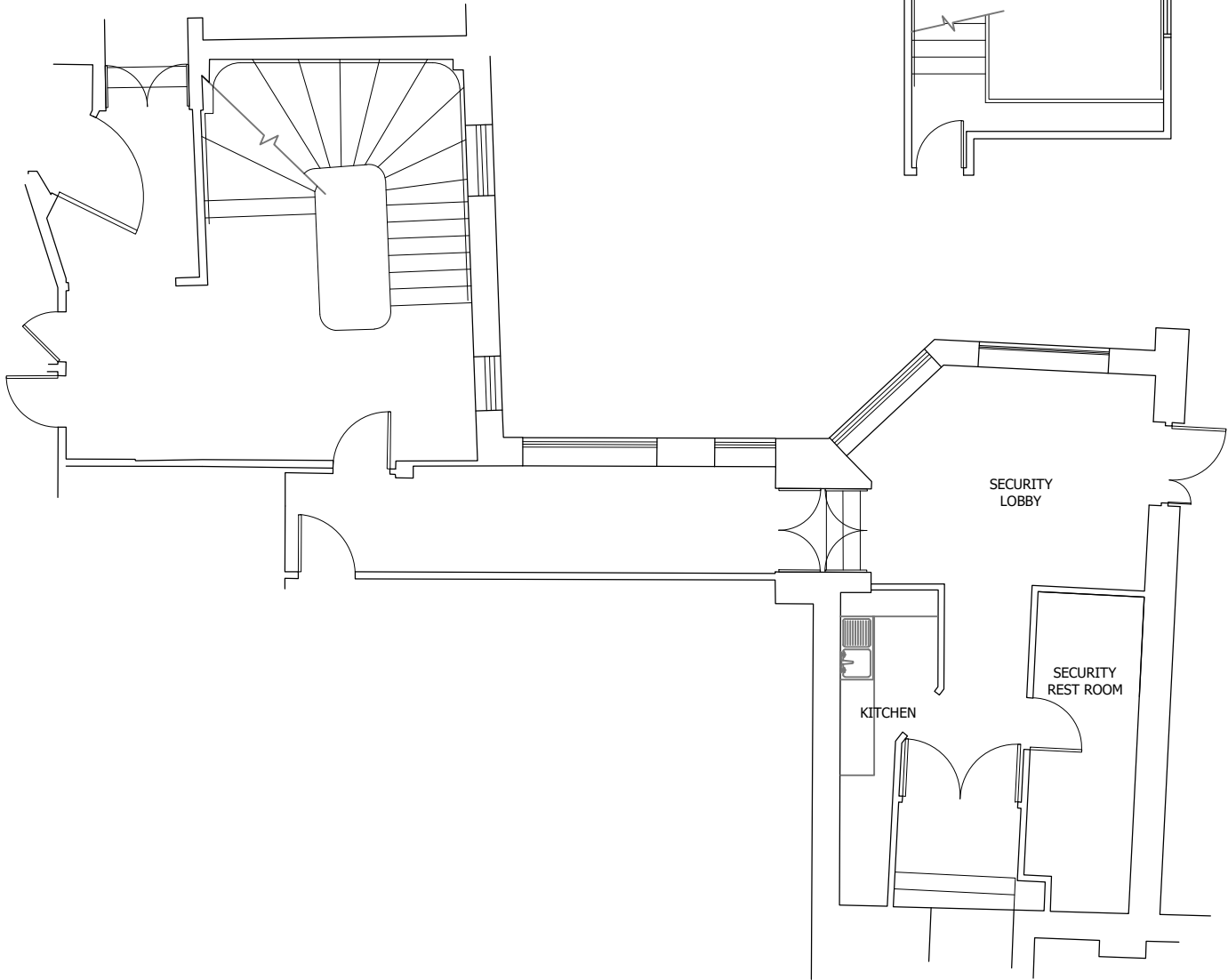
SECOND FLOOR
