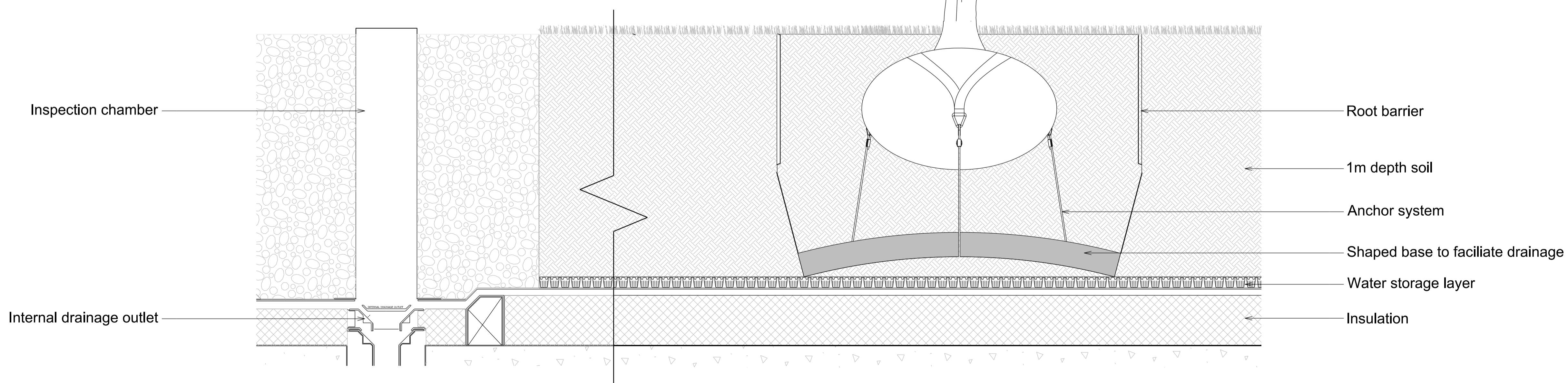
01 Typical raised garden section 1:50
