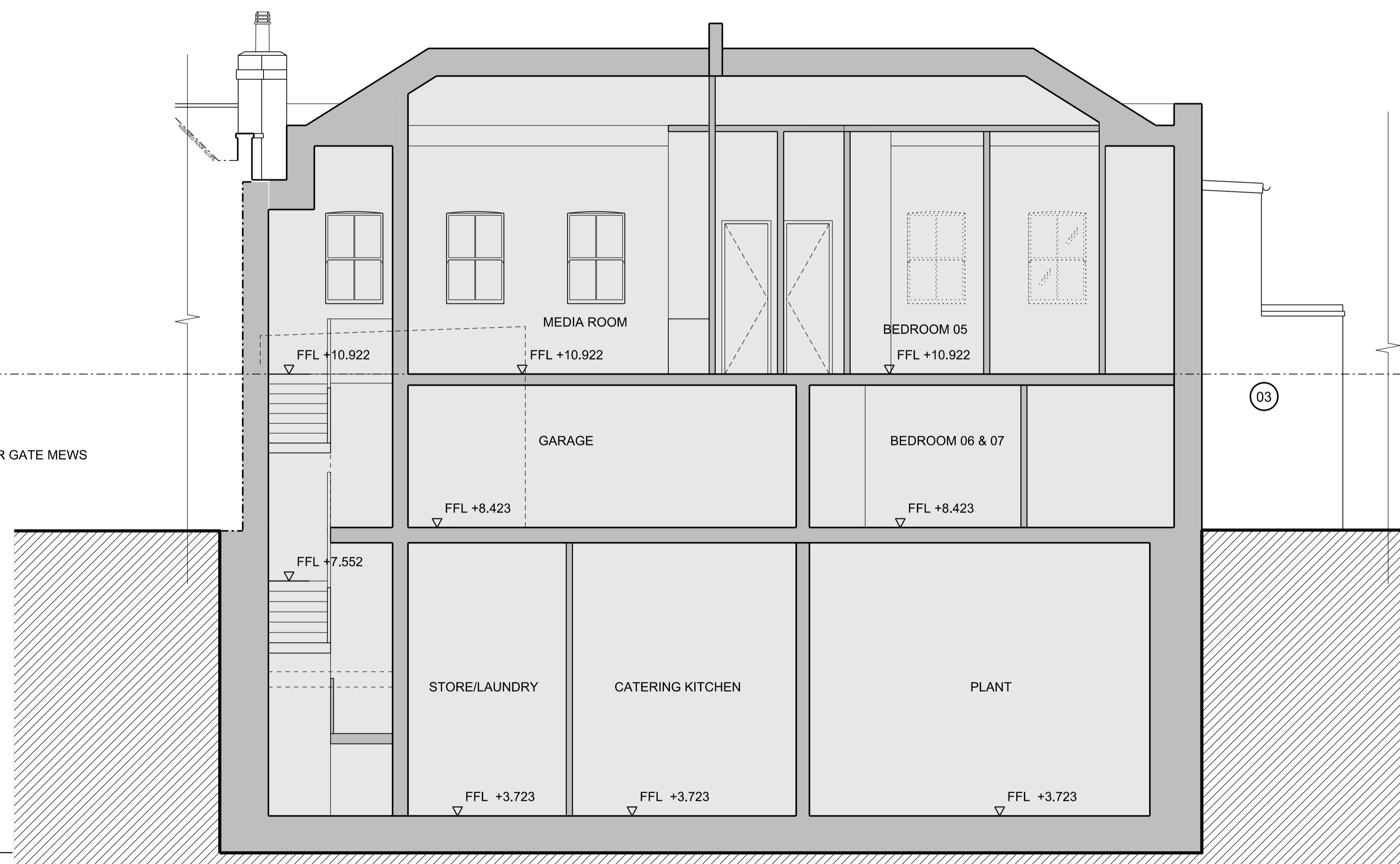
01 Proposed section E 1:50
