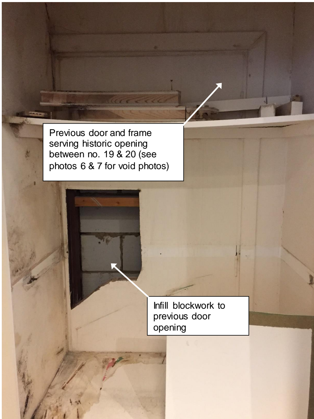
2. View of proposed door location from no. 19 Lincoln's Inn Fields. Previous door/frame and infill blockwork visible.
