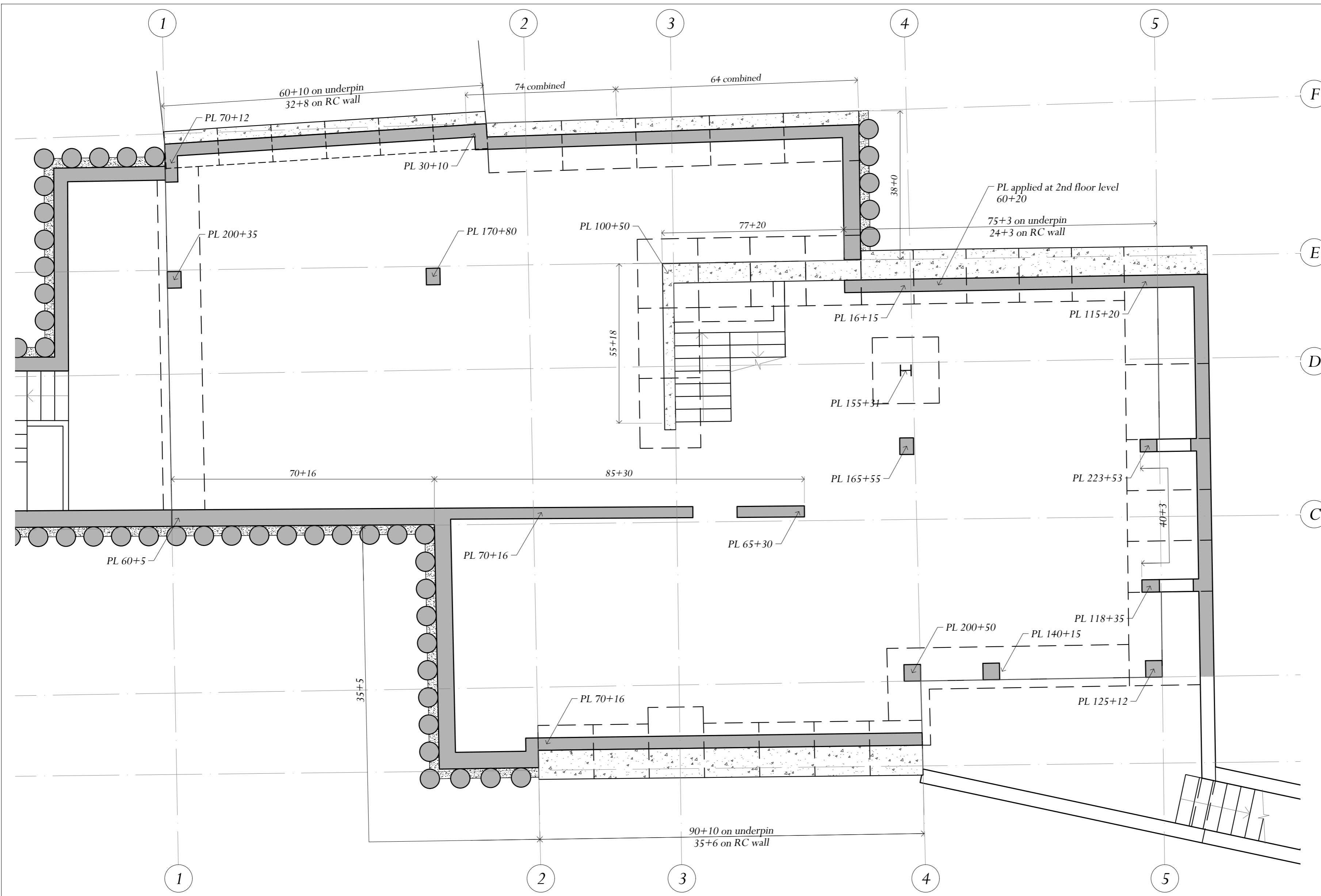
BASEMENT PLAN Scale: 1:50
