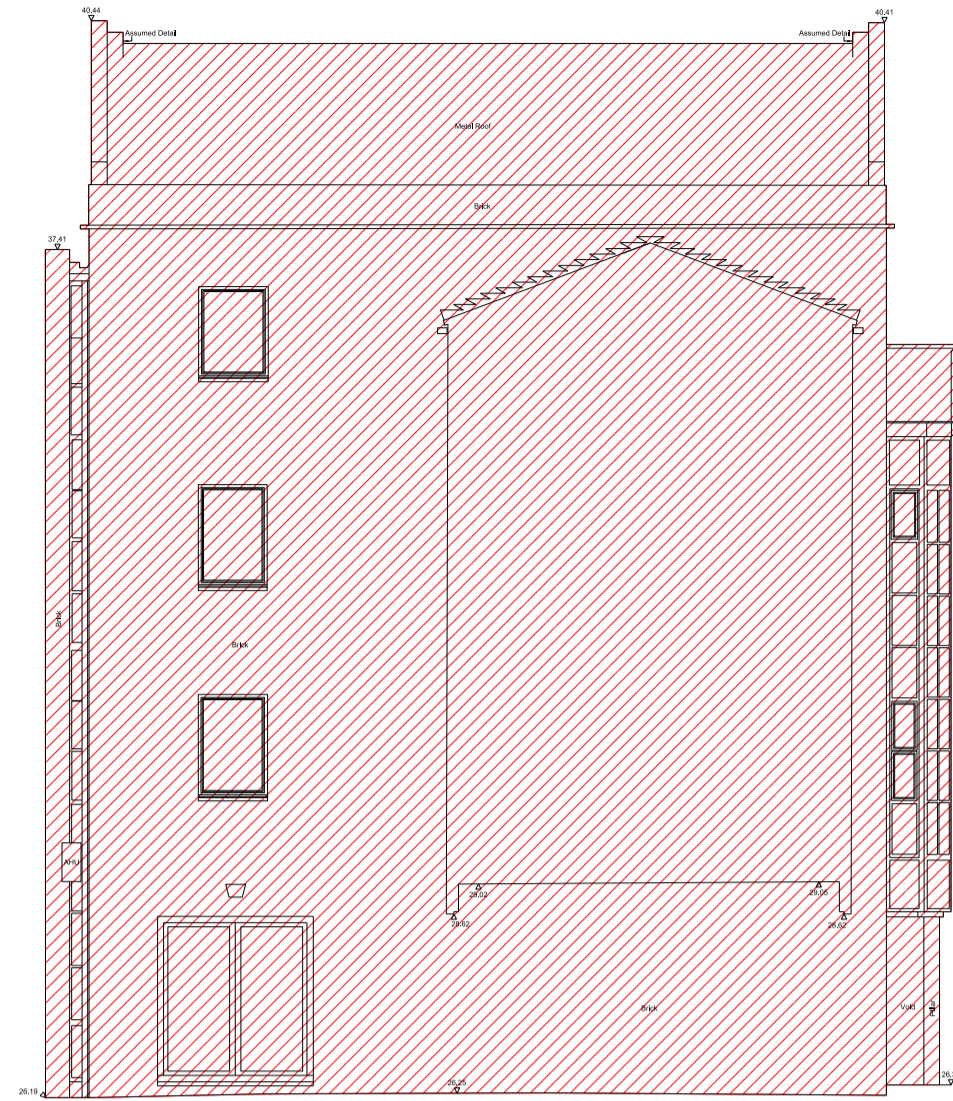
West Elevation (Internal)
