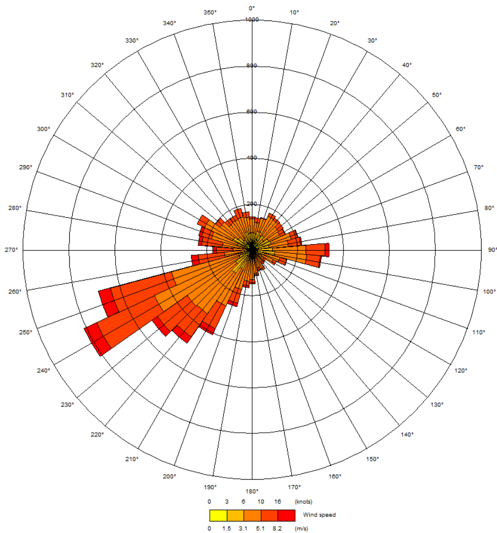
Wind Rose – London City Airport
