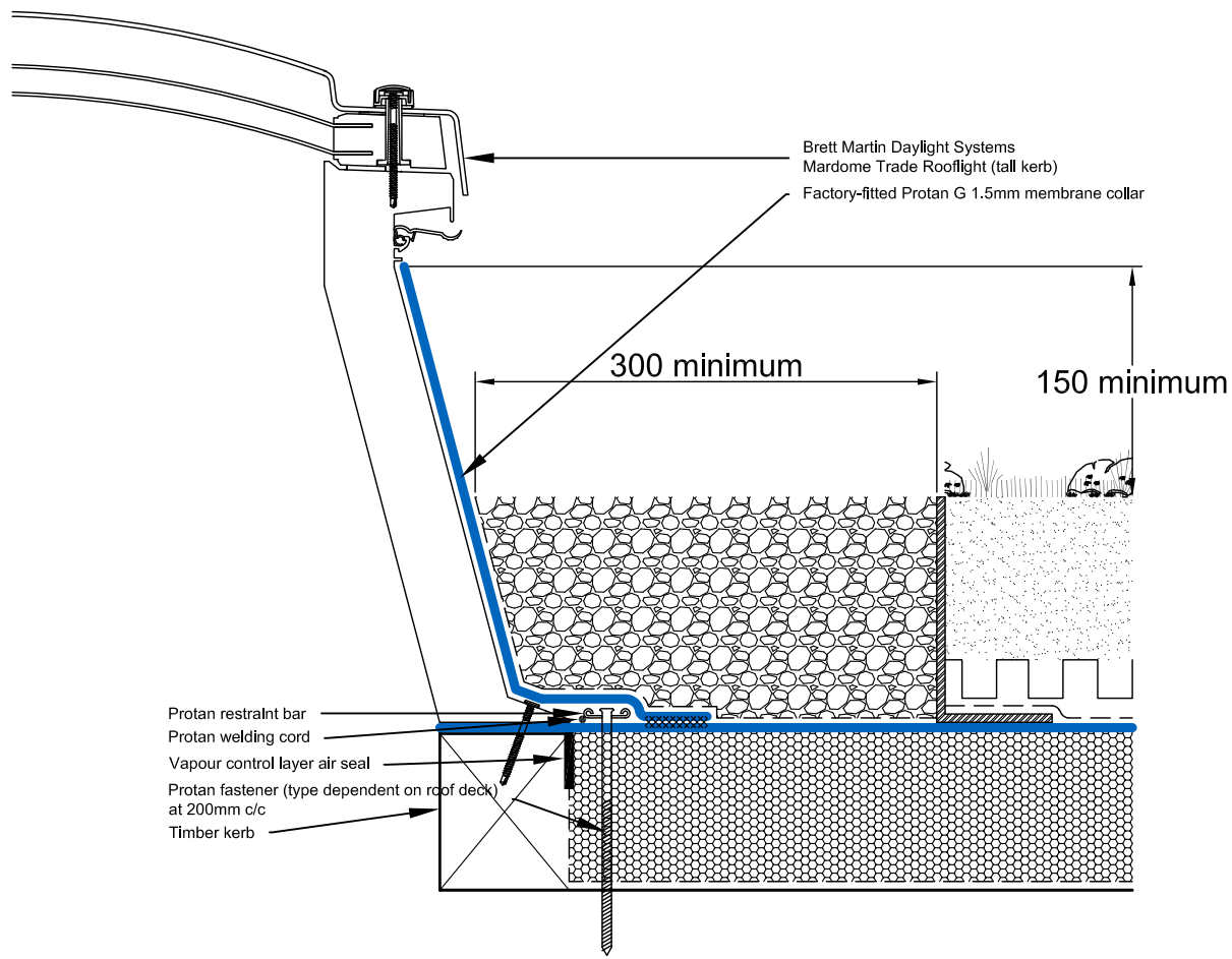
RL.GRE.W.001 PROTAN GREEN ROOF SYSTEM Rooflight Detail Warm roof construction
