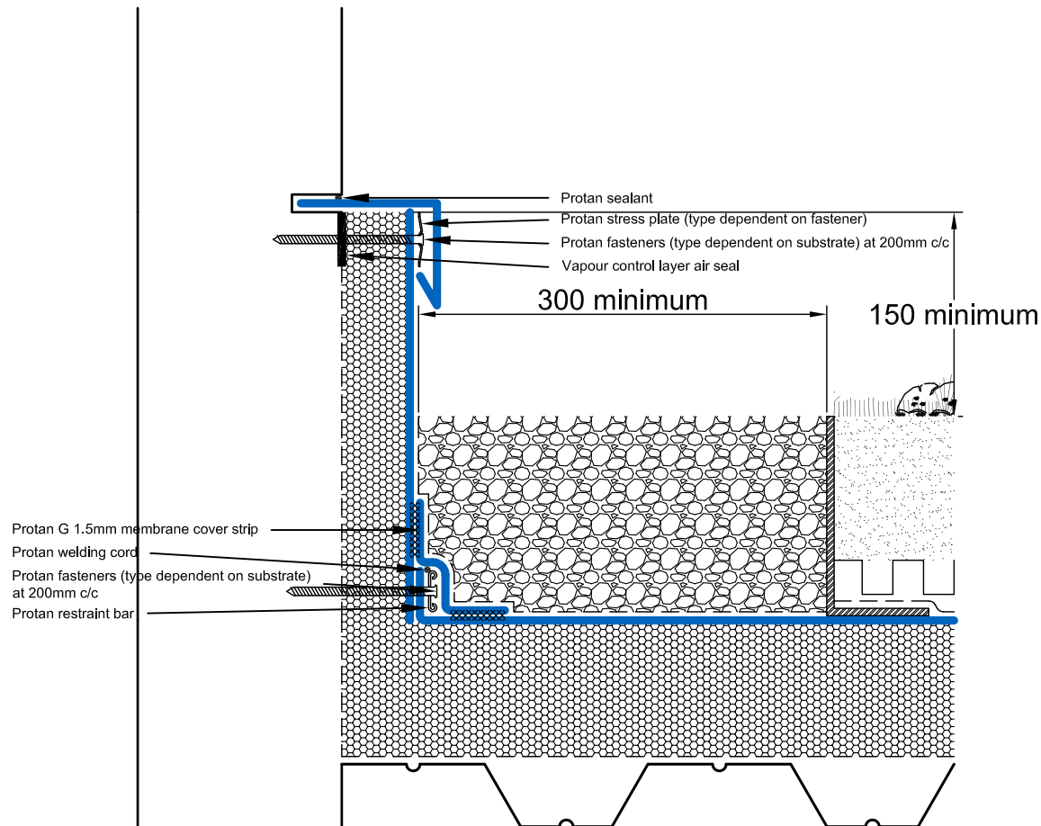
WF.GRE.W.001 PROTAN GREEN ROOF SYSTEM Wall Flashing Detail 1 Warm roof construction
