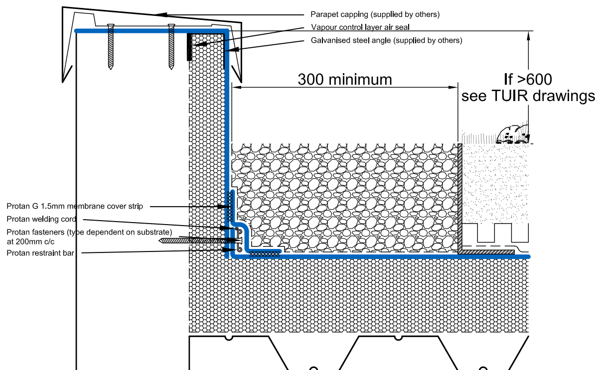
PC.GRE.W.001 PROTAN GREEN ROOF SYSTEM Parapet Capping Detail 1 Warm roof construction
