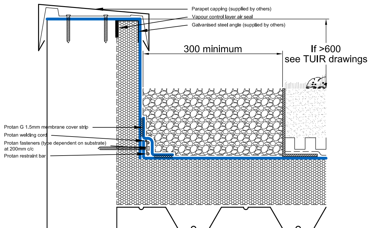
PR.GRE.W.001 PROTAN GREEN ROOF SYSTEM Perimeter Restraint into Up-stand Detail Warm roof construction
