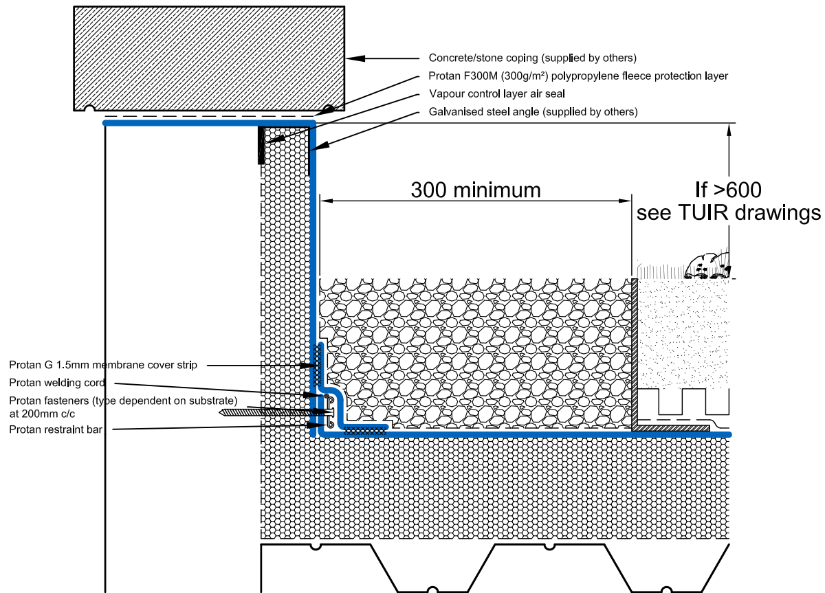
PC.GRE.W.003 PROTAN GREEN ROOF SYSTEM Parapet Capping Detail 3 Warm roof construction
