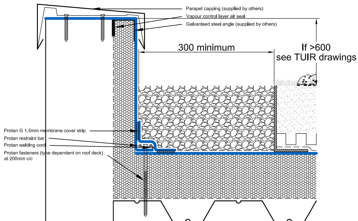
PR.GRE.W.002 PROTAN GREEN ROOF SYSTEM Perimeter Restraint into Roof Deck Detail Warm roof construction
