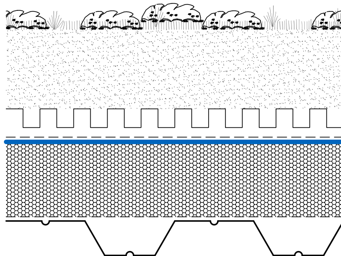
GRE.W.001 PROTAN GREEN ROOF SYSTEM Warm roof construction
