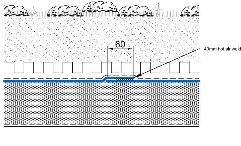
GRE.SL.W.001 PROTAN GREEN ROOF SYSTEM Side Lap Detail Warm roof construction
