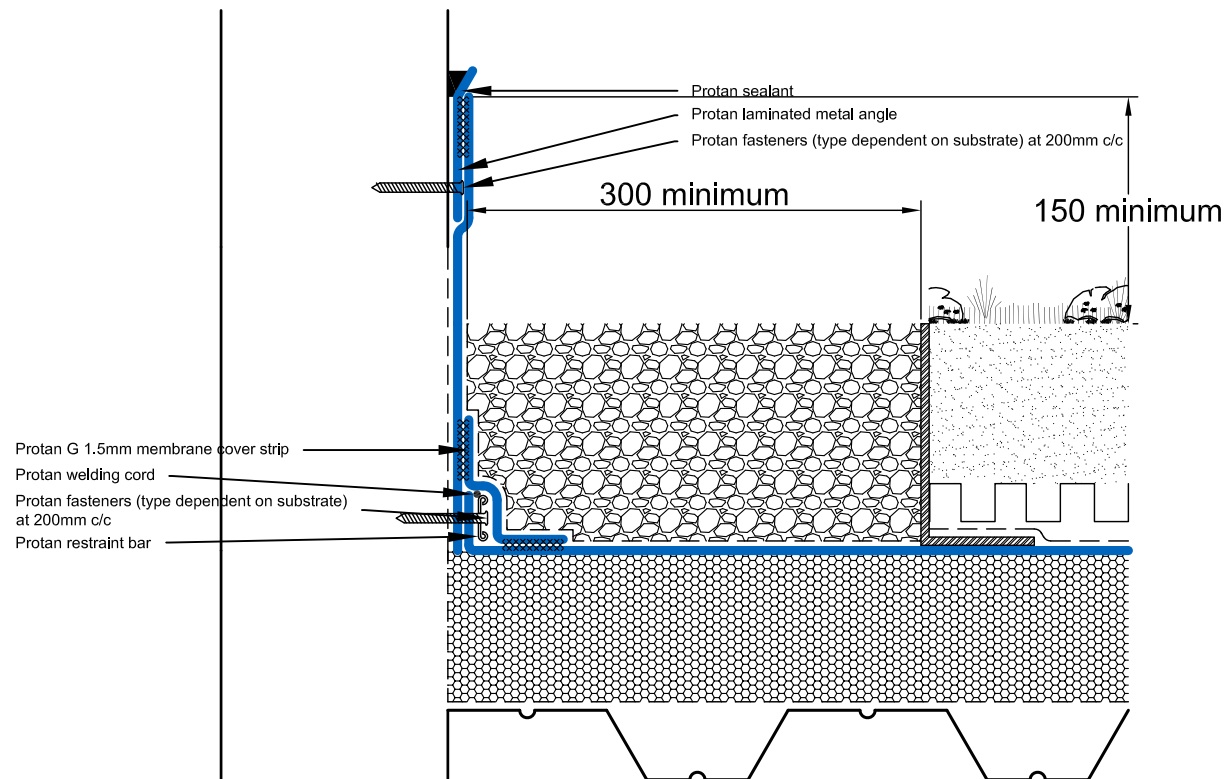
WF.GRE.W.003 PROTAN GREEN ROOF SYSTEM Wall Flashing Detail 3 Warm roof construction
