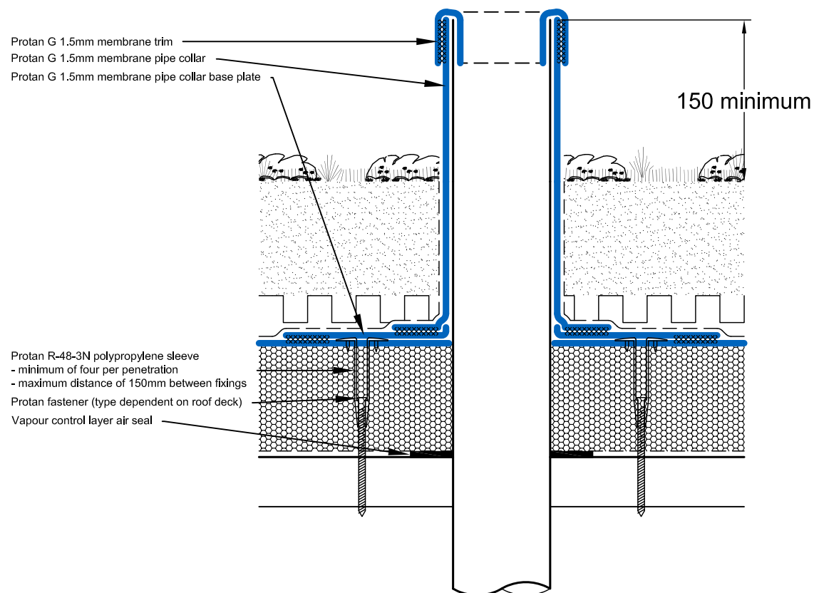
PP.GRE.W.001 PROTAN GREEN ROOF SYSTEM Pipe Penetration Detail (Closed) Warm roof construction
