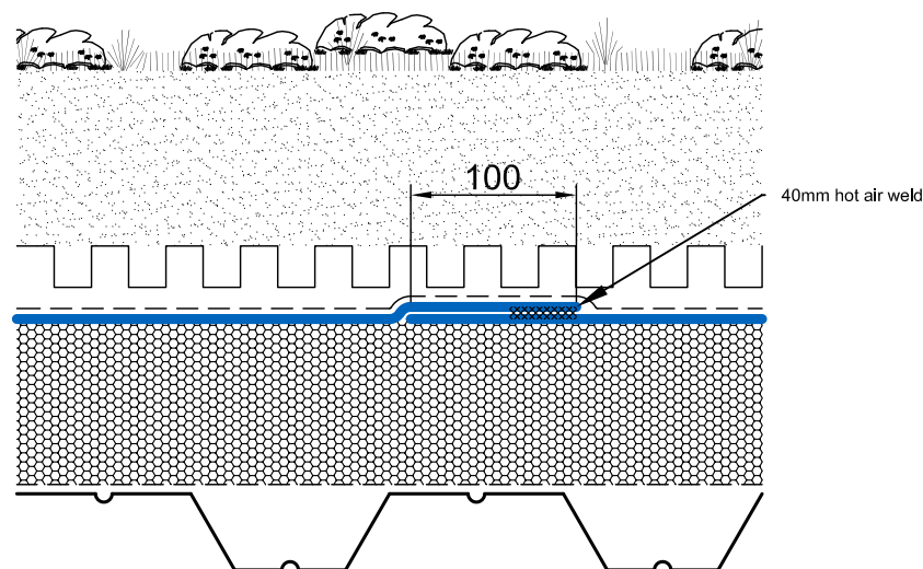
GRE.EL.W.001 PROTAN GREEN ROOF SYSTEM End Lap Detail 1 Warm roof construction
