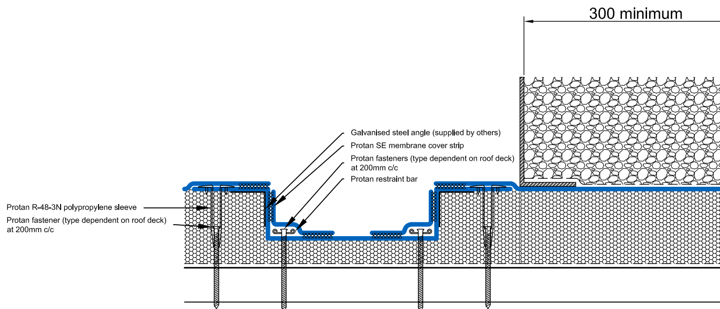
BG.GRE.W.001 PROTAN GREEN ROOF SYSTEM Box Gutter Detail Warm roof construction
