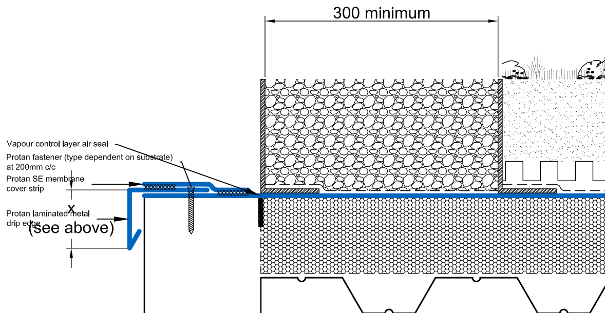
DE.GRE.W.001 PROTAN GREEN ROOF SYSTEM Drip Edge Detail Warm roof construction
