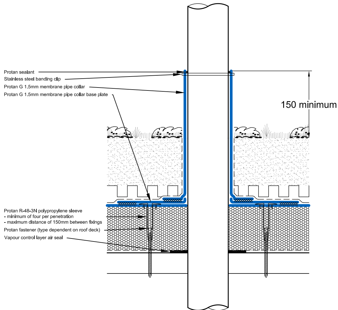
PP.GRE.W.002 PROTAN GREEN ROOF SYSTEM Pipe Penetration Detail (Continuous) Warm roof construction
