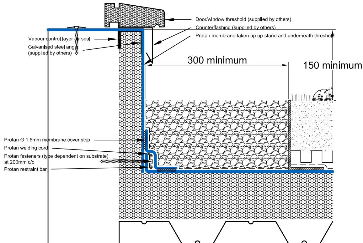
DWT.GRE.W.001 PROTAN GREEN ROOF SYSTEM Door/Window Threshold Detail Warm roof construction
