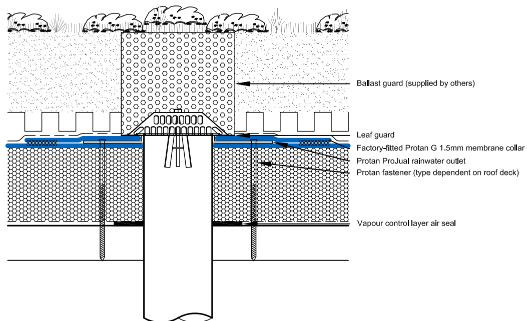
RO.GRE.W.001 PROTAN GREEN ROOF SYSTEM Rainwater Outlet Detail Warm roof construction
