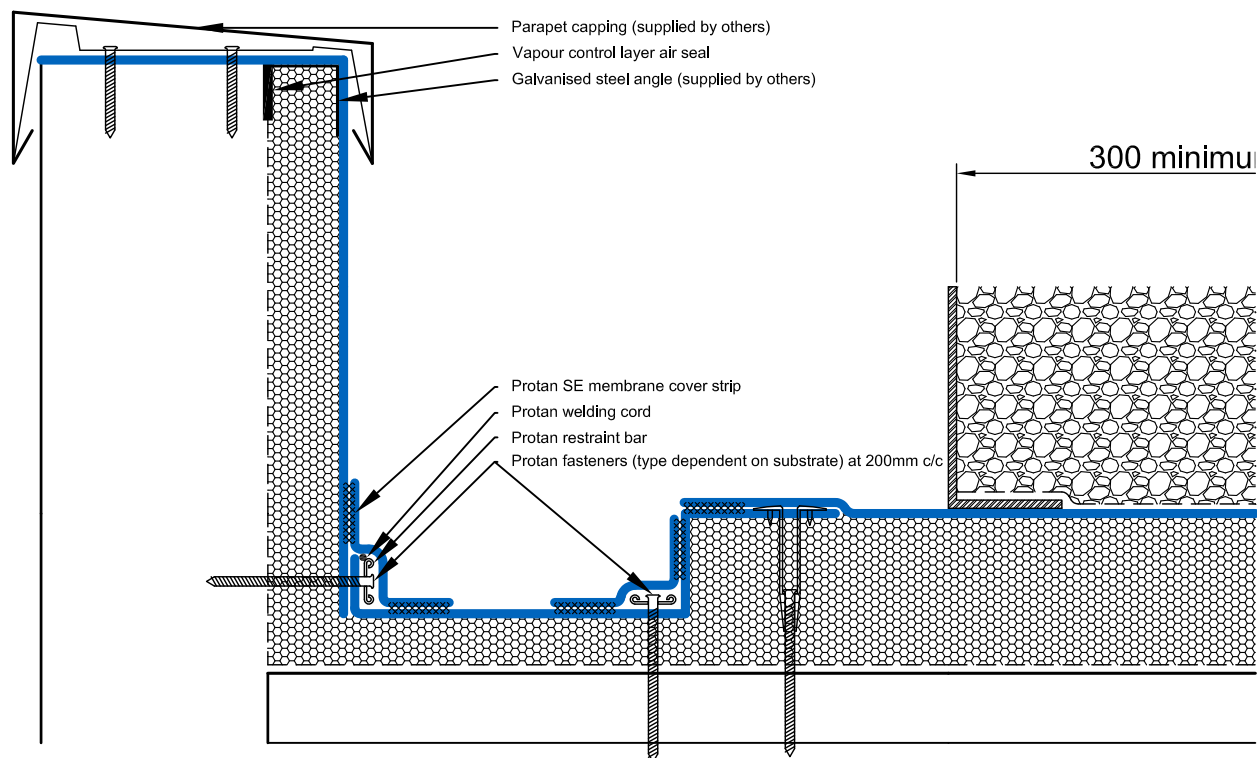
PG.GRE.W.001 PROTAN GREEN ROOF SYSTEM Perimeter Gutter Detail Warm roof construction
