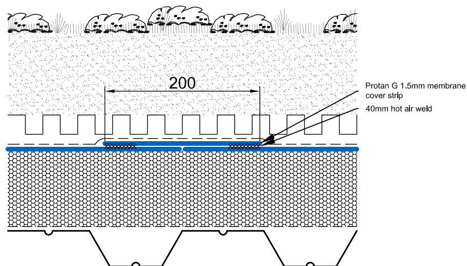
GRE.EL.W.002 PROTAN PREFABRICATED GREEN ROOF SYSTEM End Lap Detail 2 Warm roof construction
