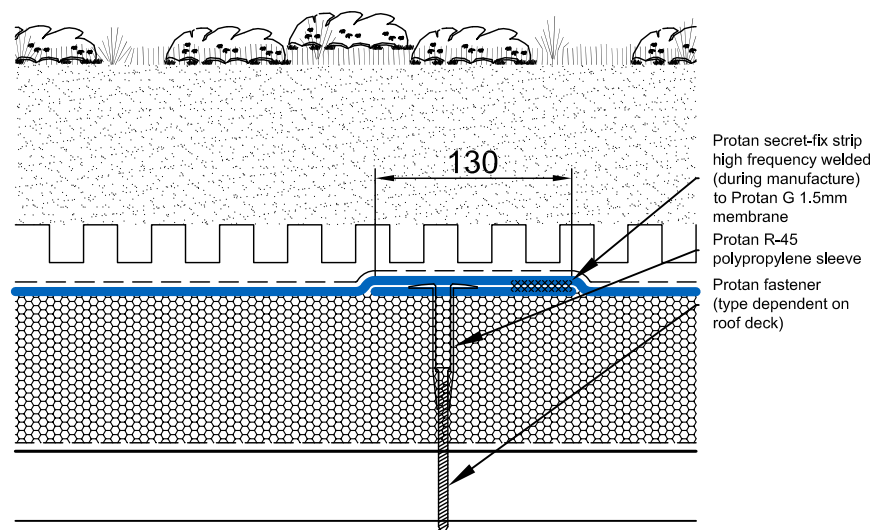
GRE.SF.W.001 PROTAN PREFABRICATED GREEN ROOF SYSTEM Secret Fix Detail Warm roof construction
