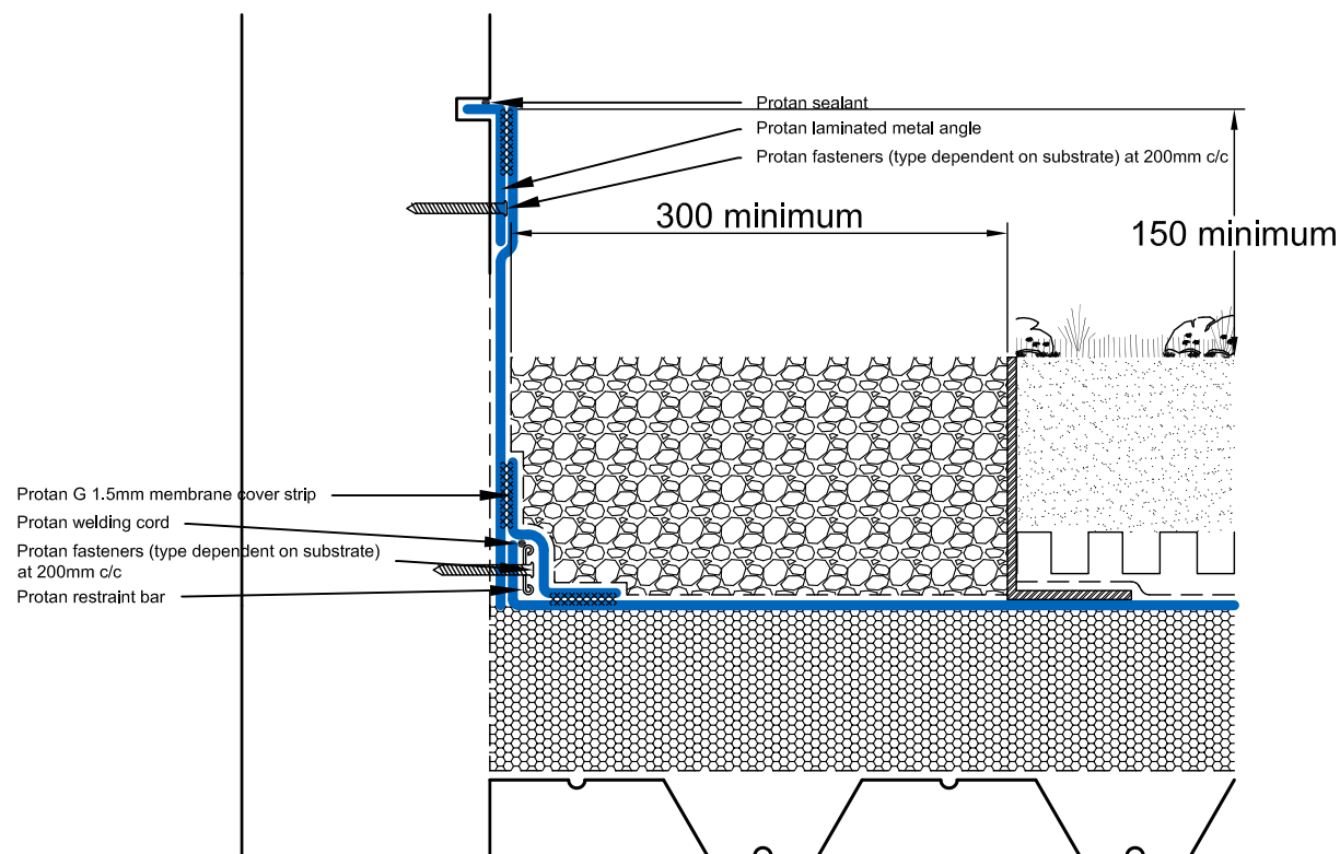
WF.GRE.W.002 PROTAN GREEN ROOF SYSTEM Wall Flashing Detail 2 Warm roof construction
