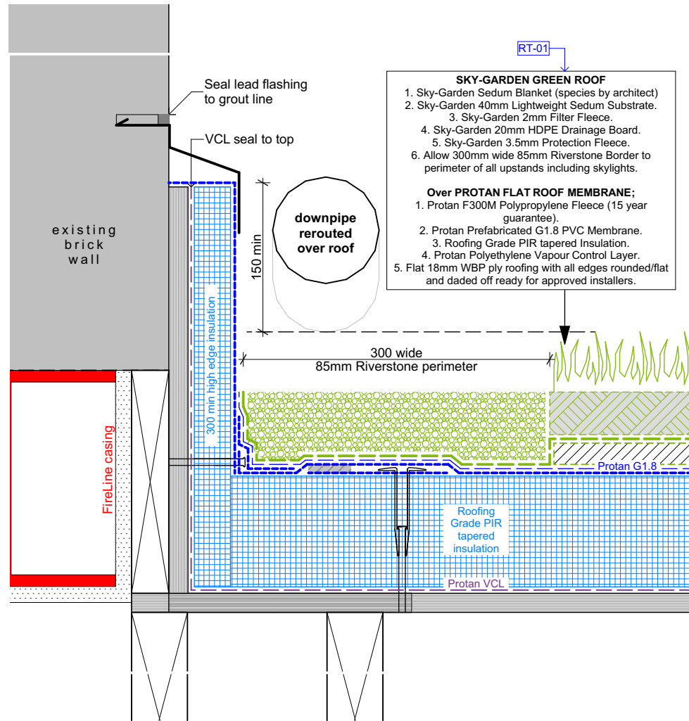
03 D-03: Living Roof to Existing Brick Wall Scale 1:5
