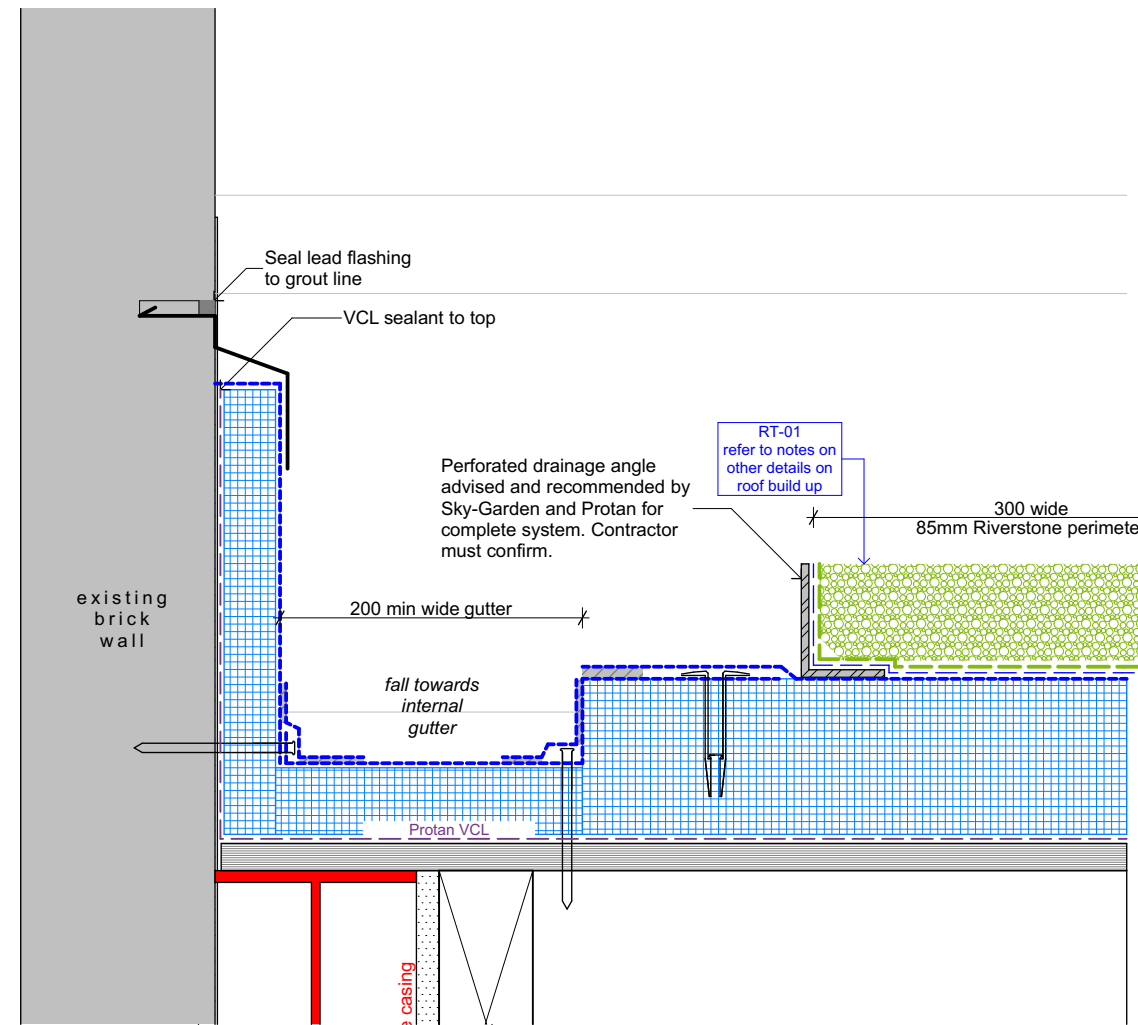
04 D-04: Living Roof - Gutter Detail to Party Wall Scale 1:5
