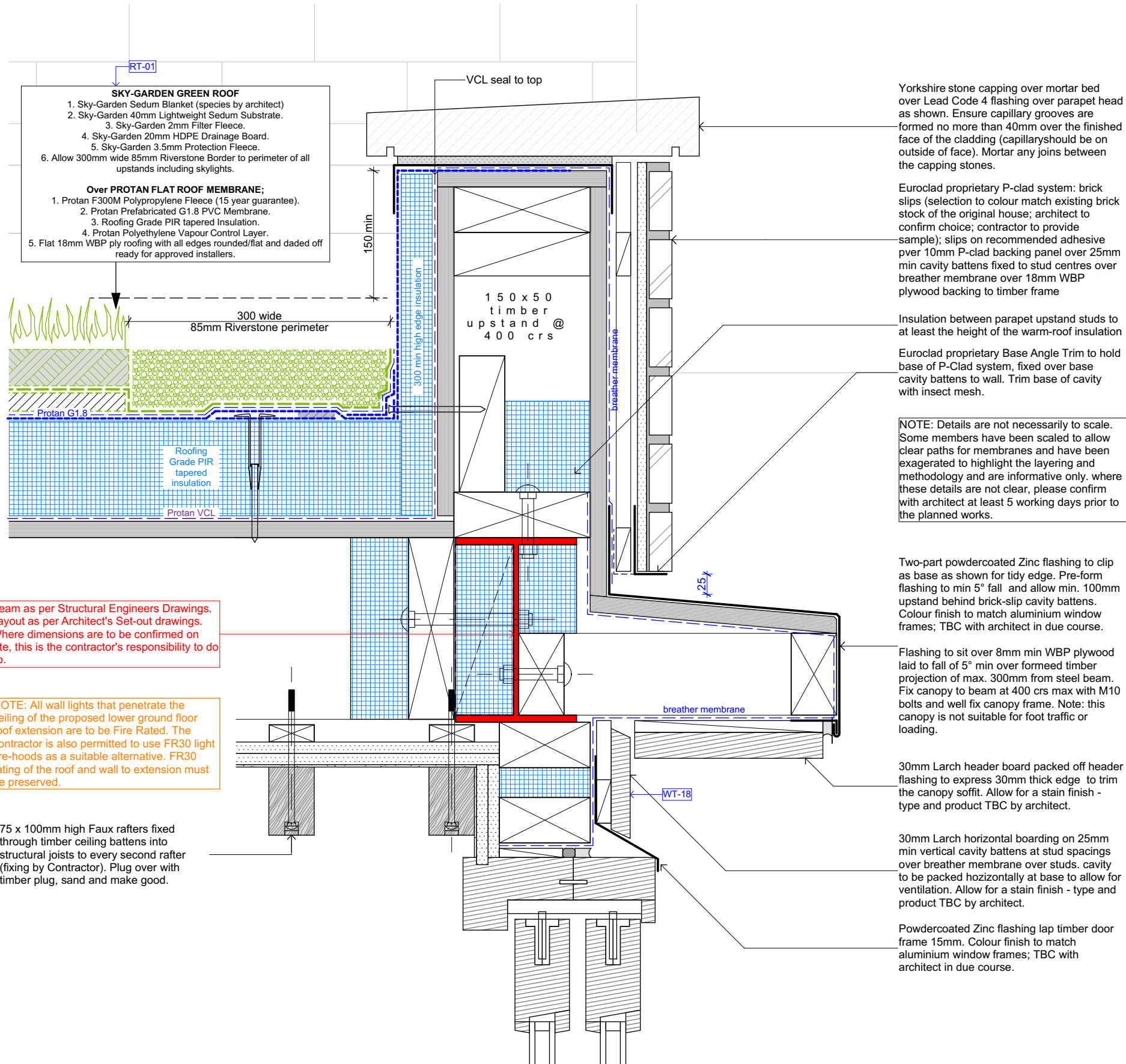
01 D-01: Living Roof Parapet Scale 1:5
