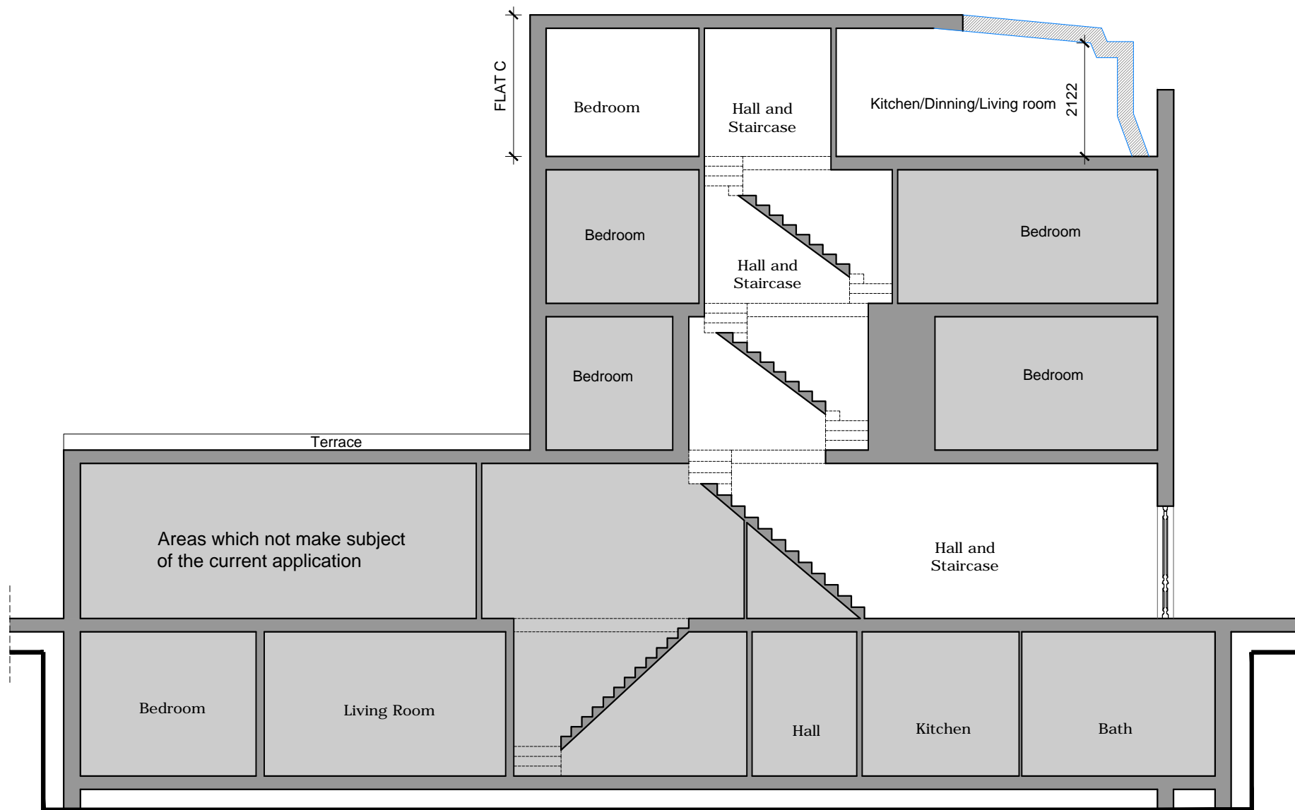
Proposed Section A-A
