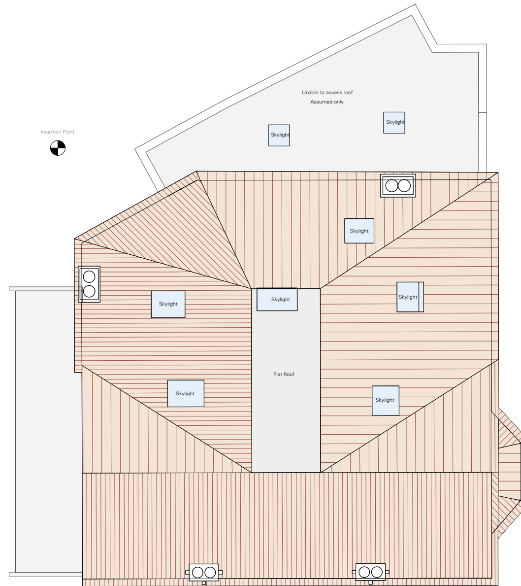
2 Roof Plan Existing 005 Scale: 1:100
