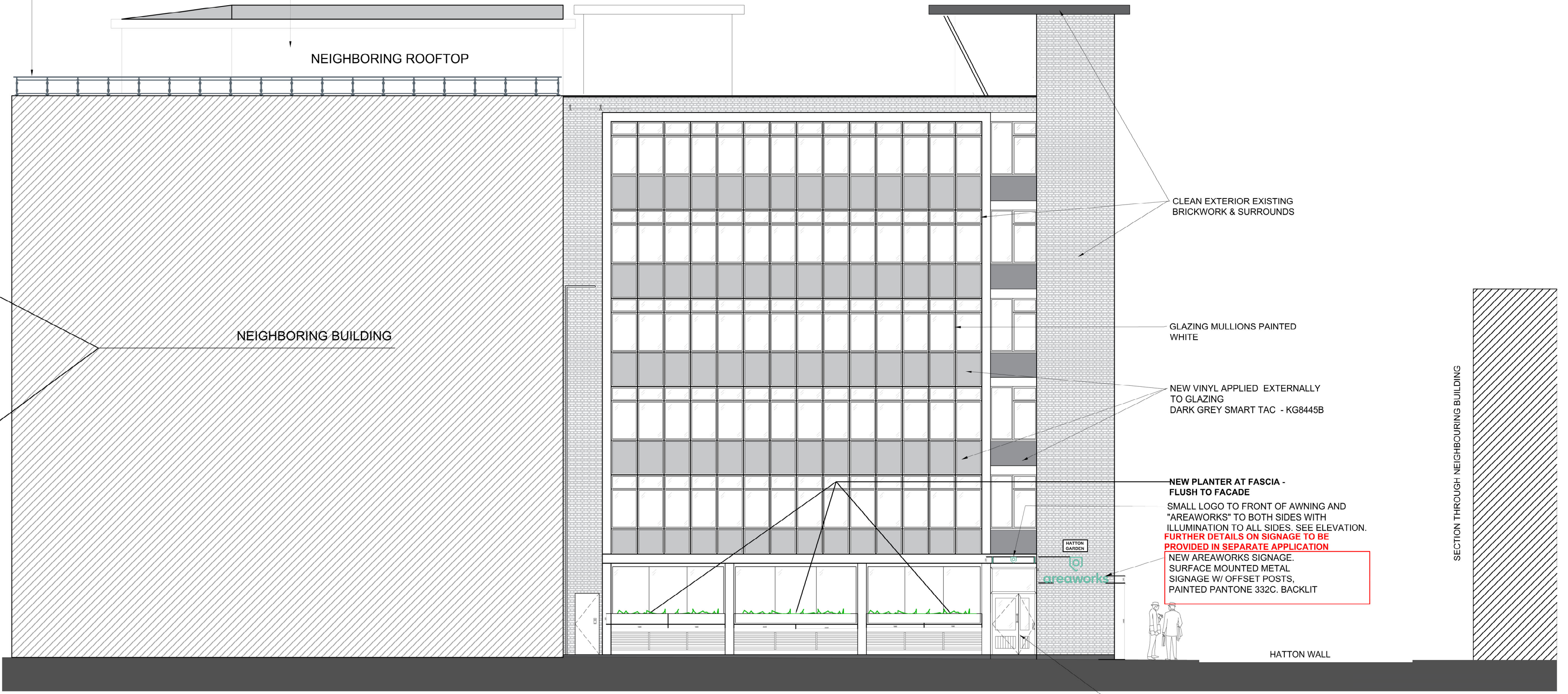
PROPOSED S/W ELEVATION - HATTON GARDEN
