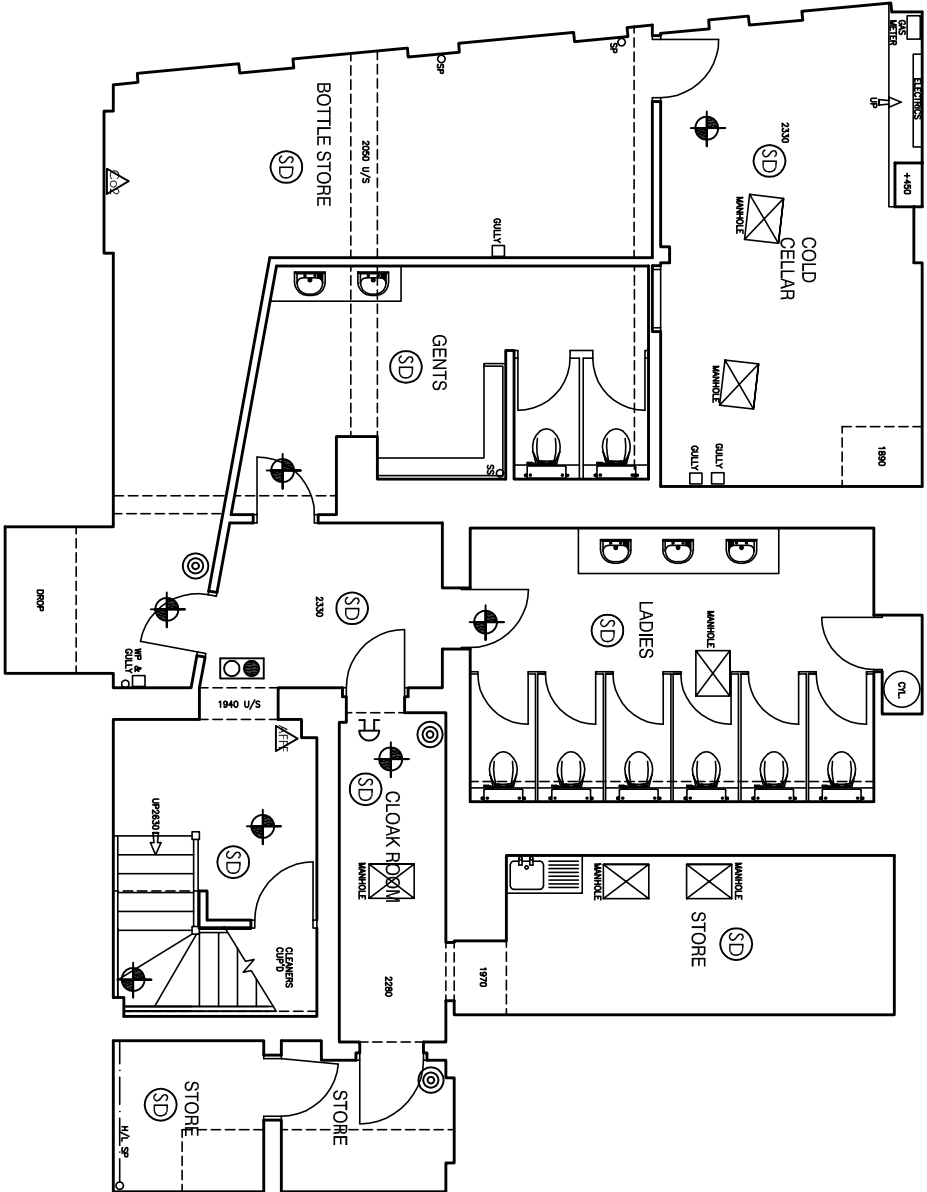
BASEMENT PLAN
