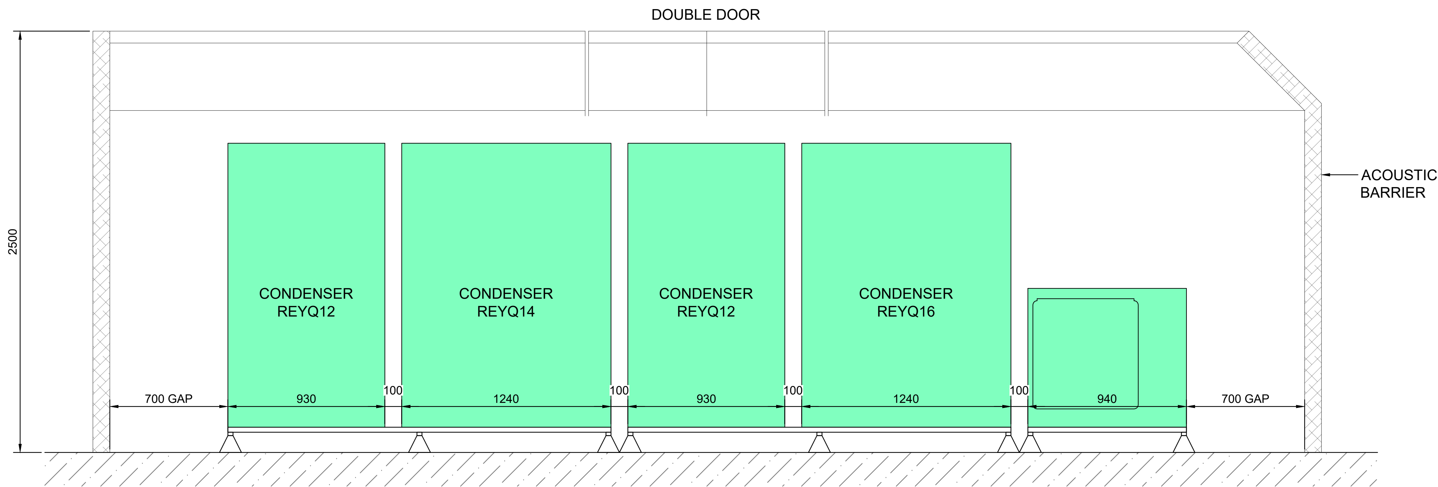
CONDENSER ELEVATION B-B
