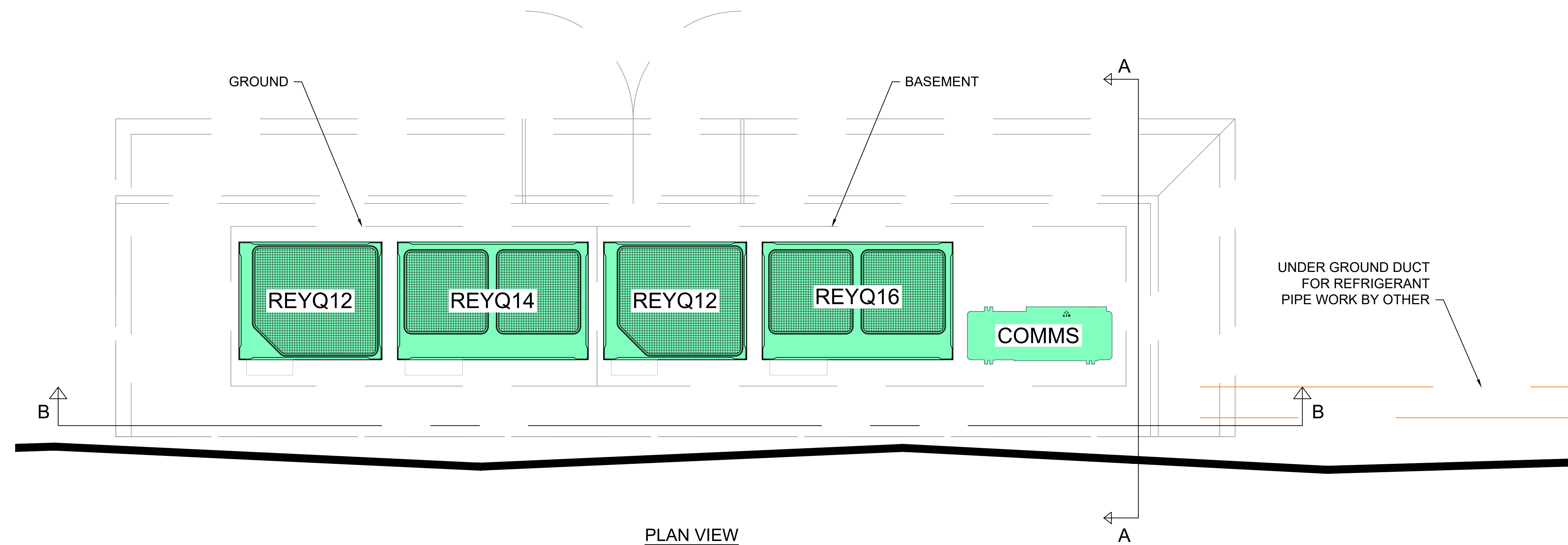
PLAN VIEW
