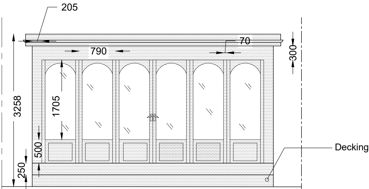
Front Elevation
