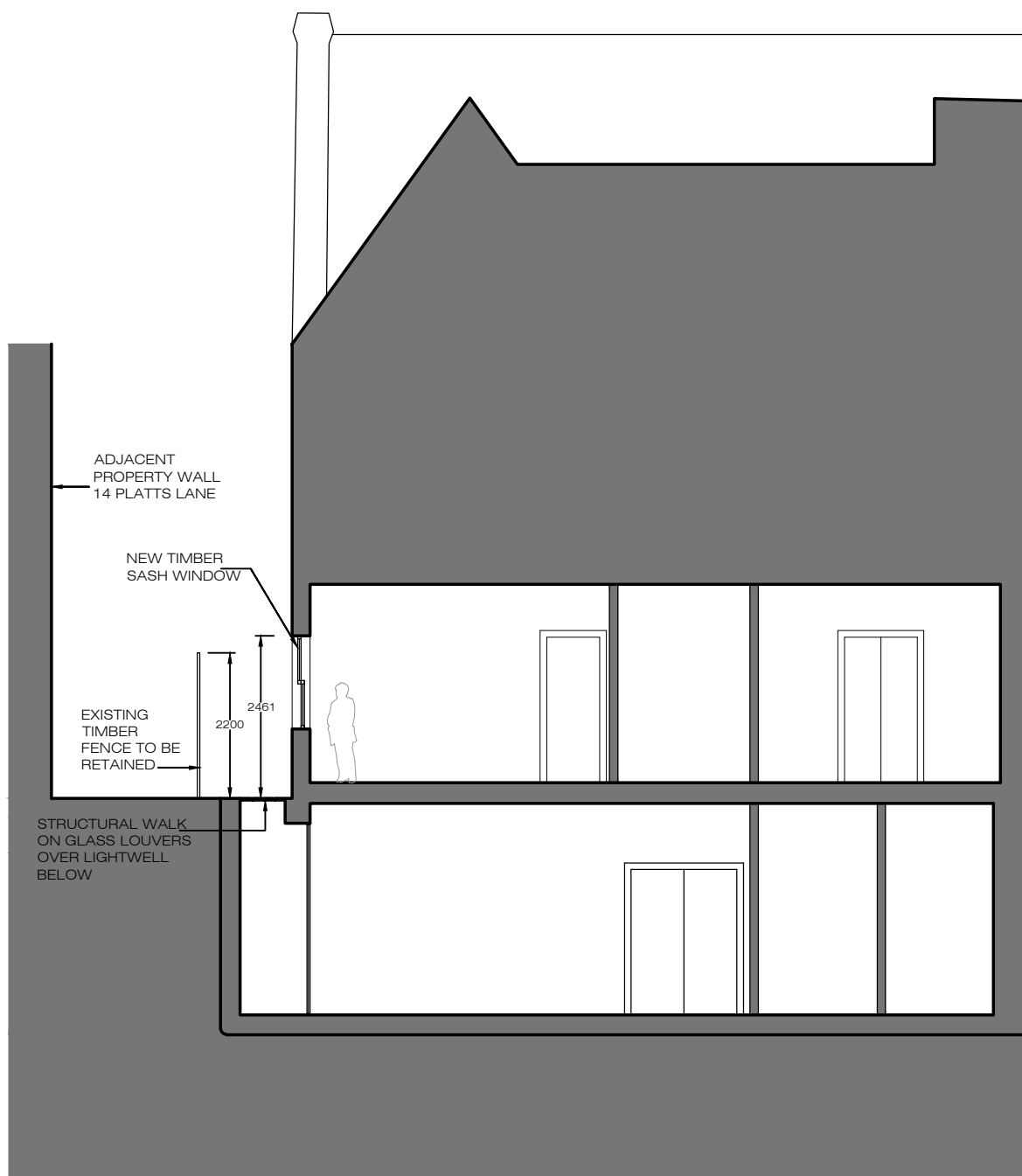
Section BB
