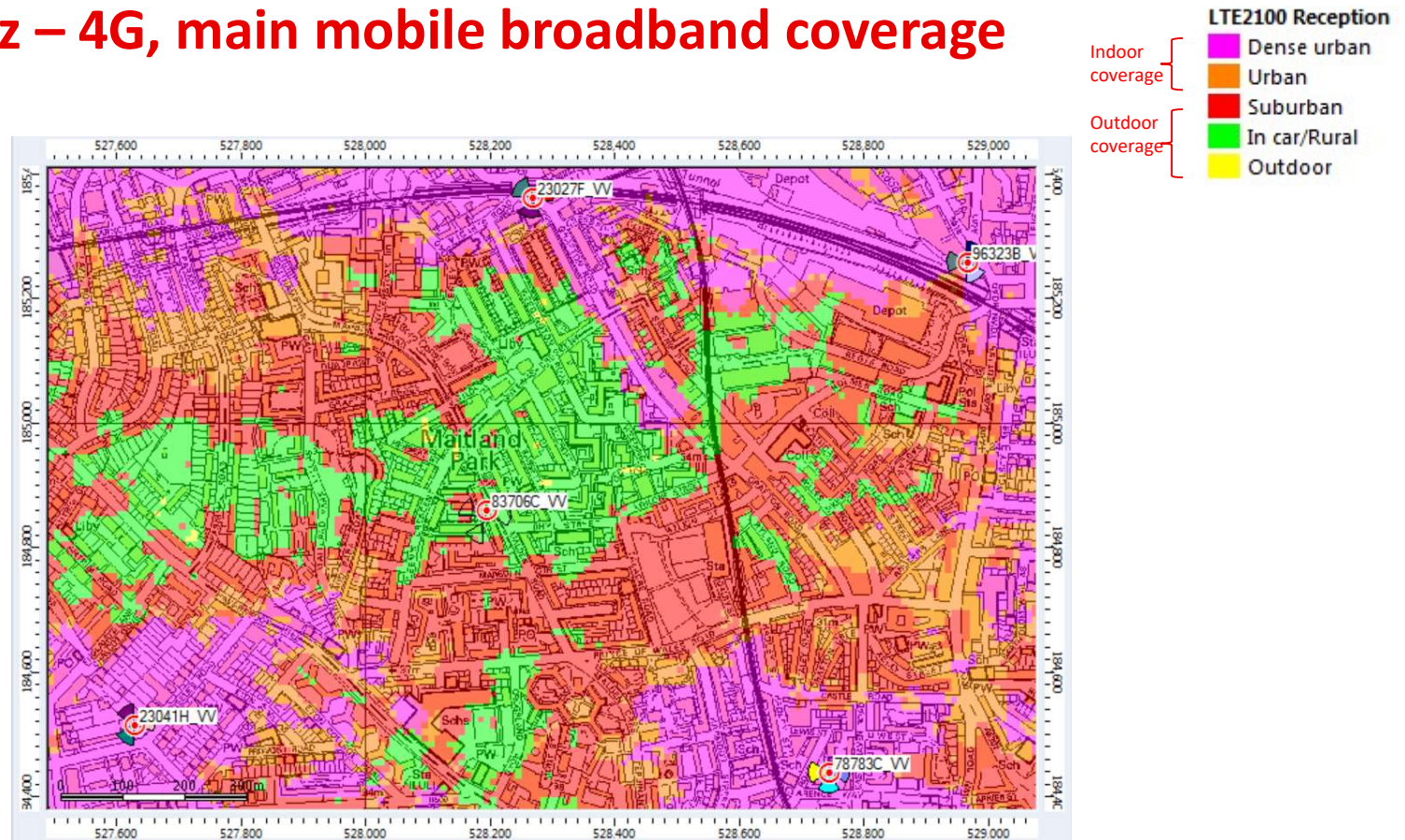
Fig. 3: Existing LTE2100MHz, main mobile broadband coverage
