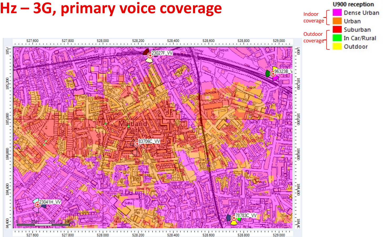
Fig. 1: Existing voice coverage
