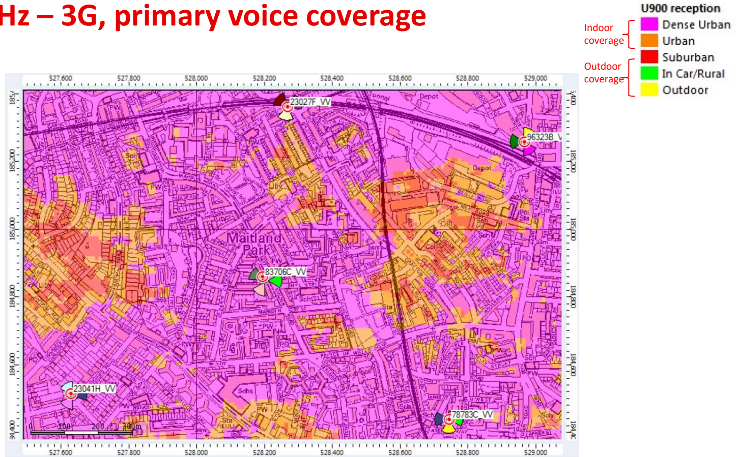
Fig. 2: Proposed voice coverage
