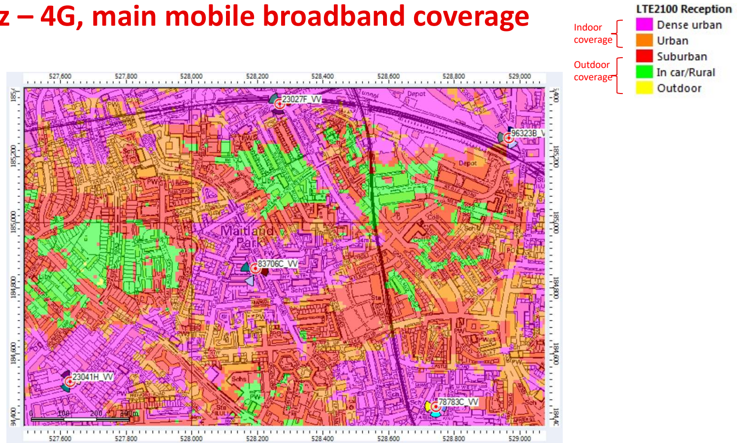
Fig 4. proposed LTE2100MHz, main mobile broadband coverage
