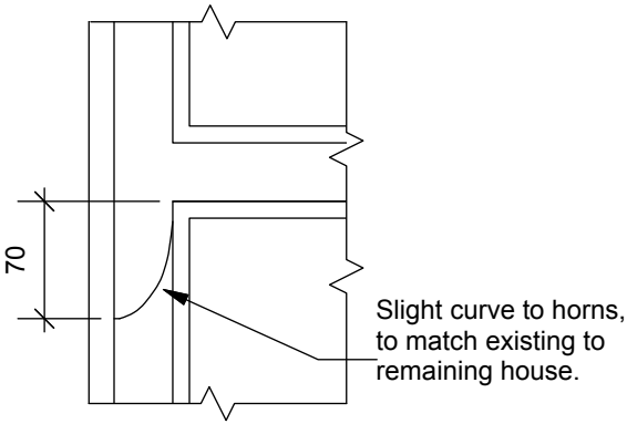
EXTERNAL HORNS TO TOP SASH (scale 1:5 @ A3)
