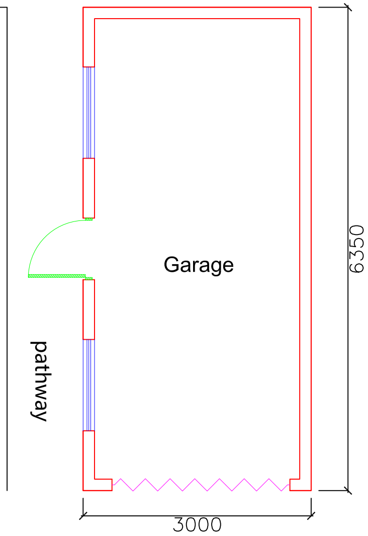
Existing Plan
