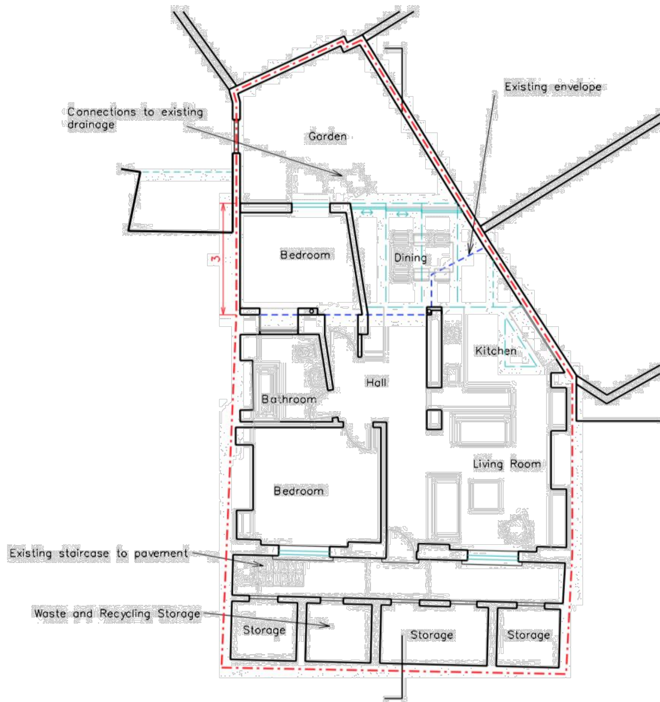
BASEMENT PLAN
