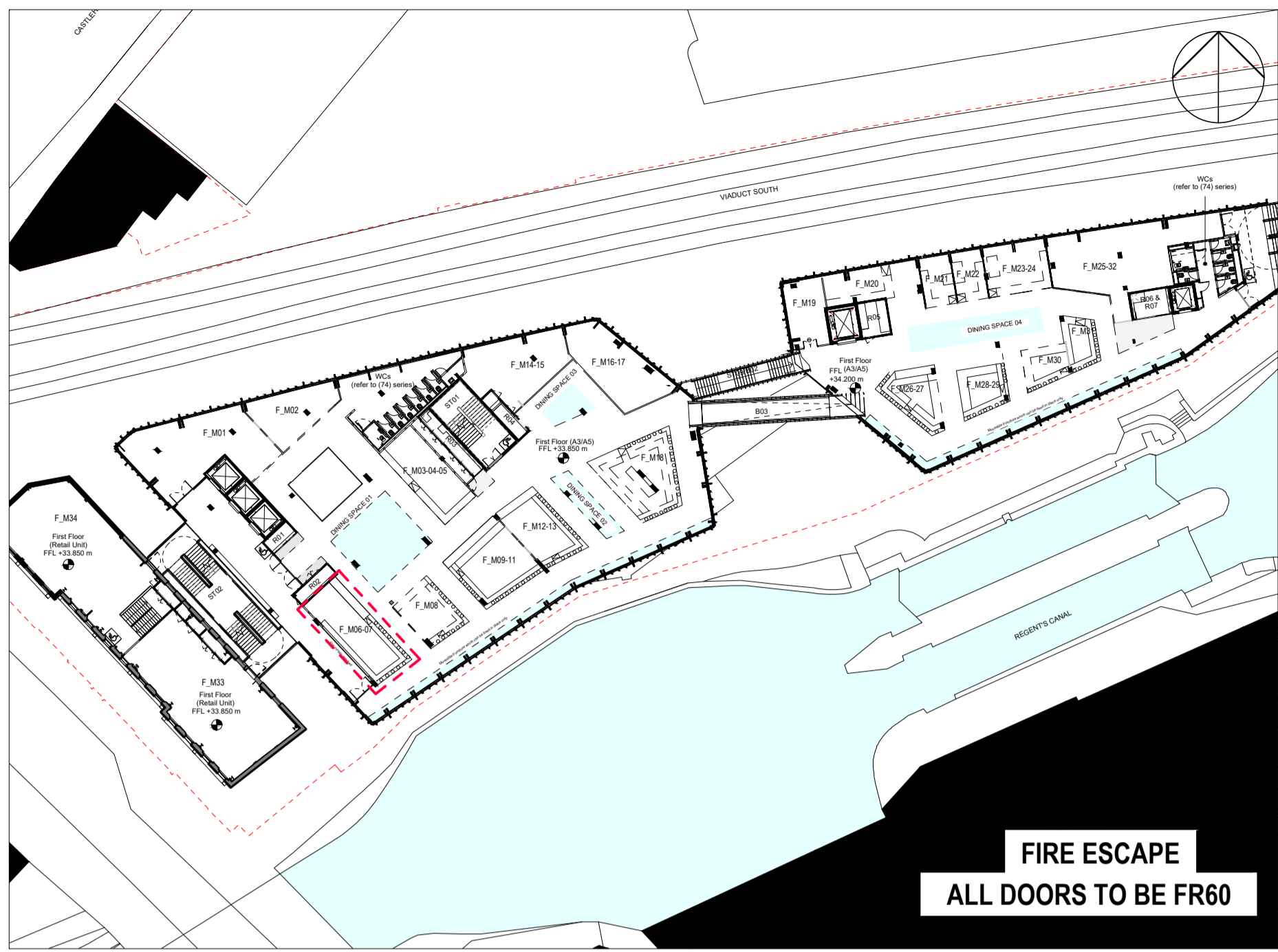
UPPER LOCK _ FIRST FLOOR PLAN SCALE 1:500
