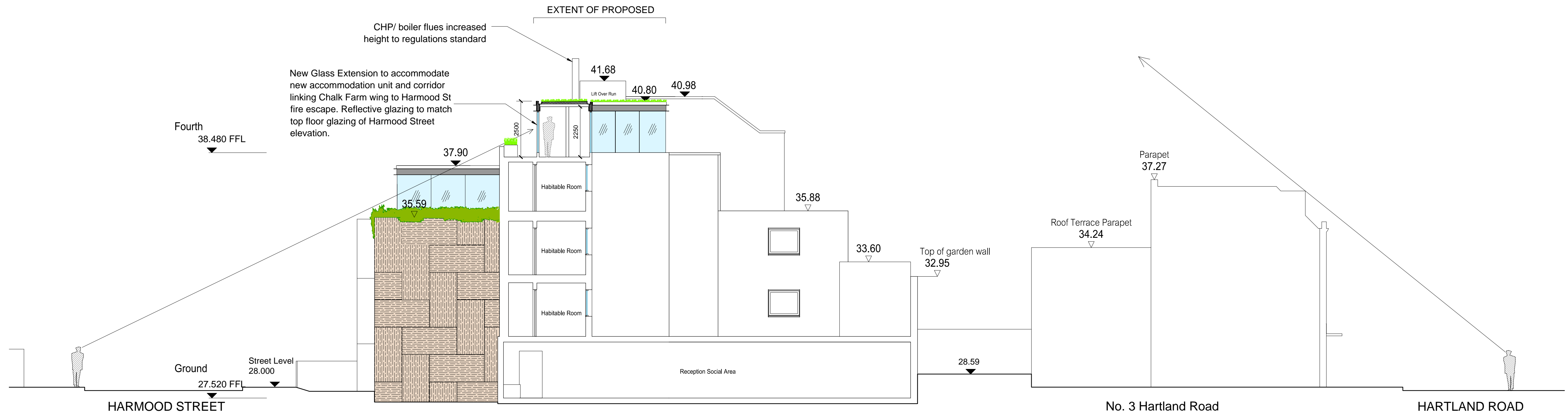
PROPOSED SECTION A-A
