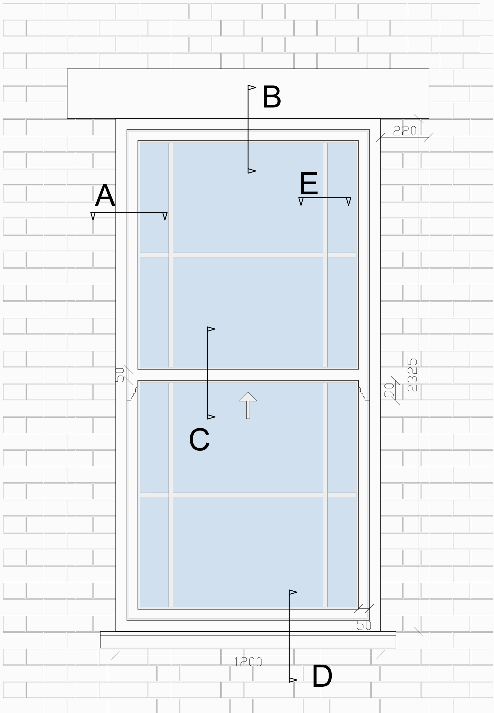
FRONT AND SIDE FIRST FLOOR'S WINDOW ELEVATION SCALE 1/10 at A3
