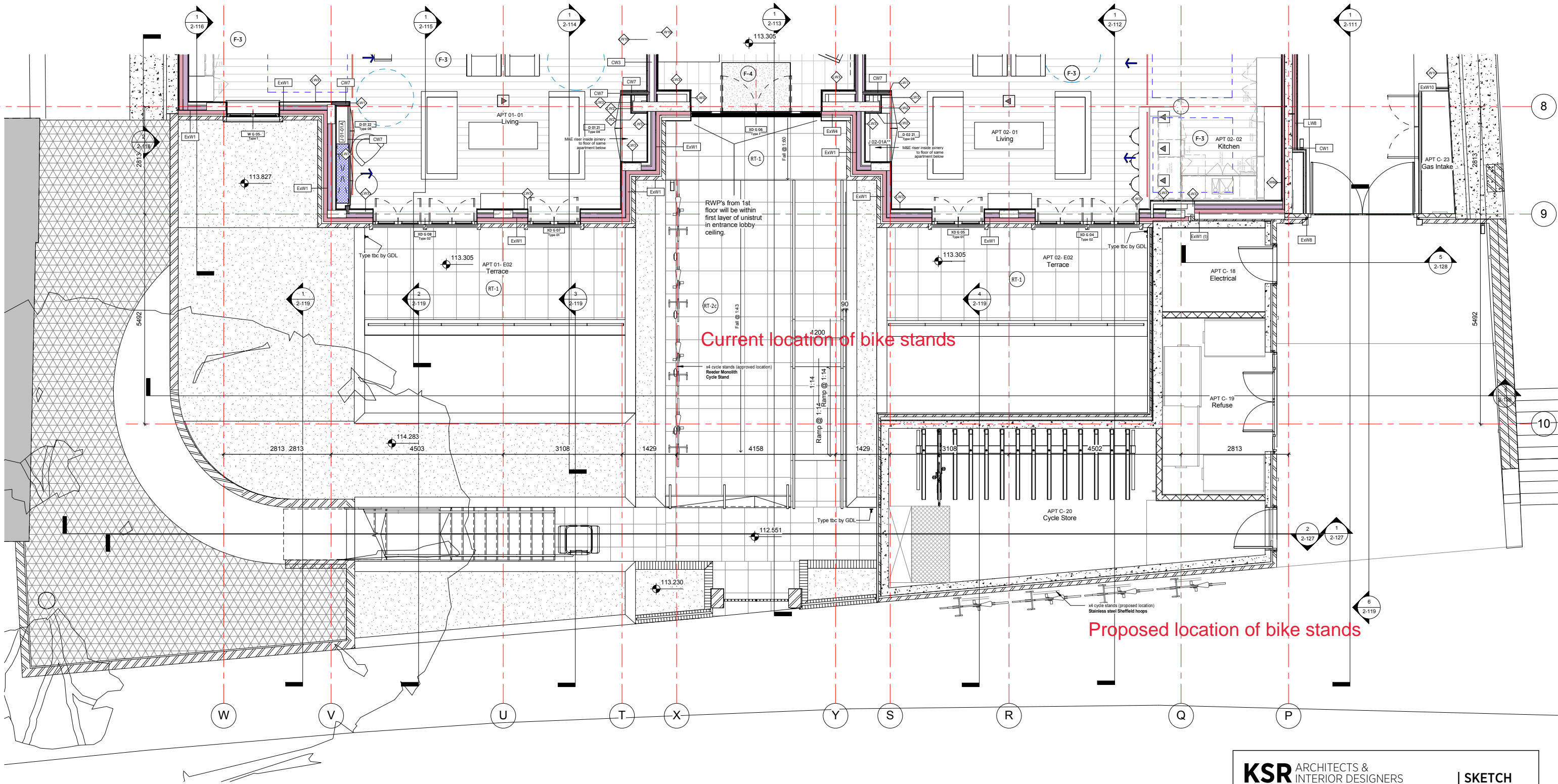
1 Level 0 South (Externals) 1 : 50
