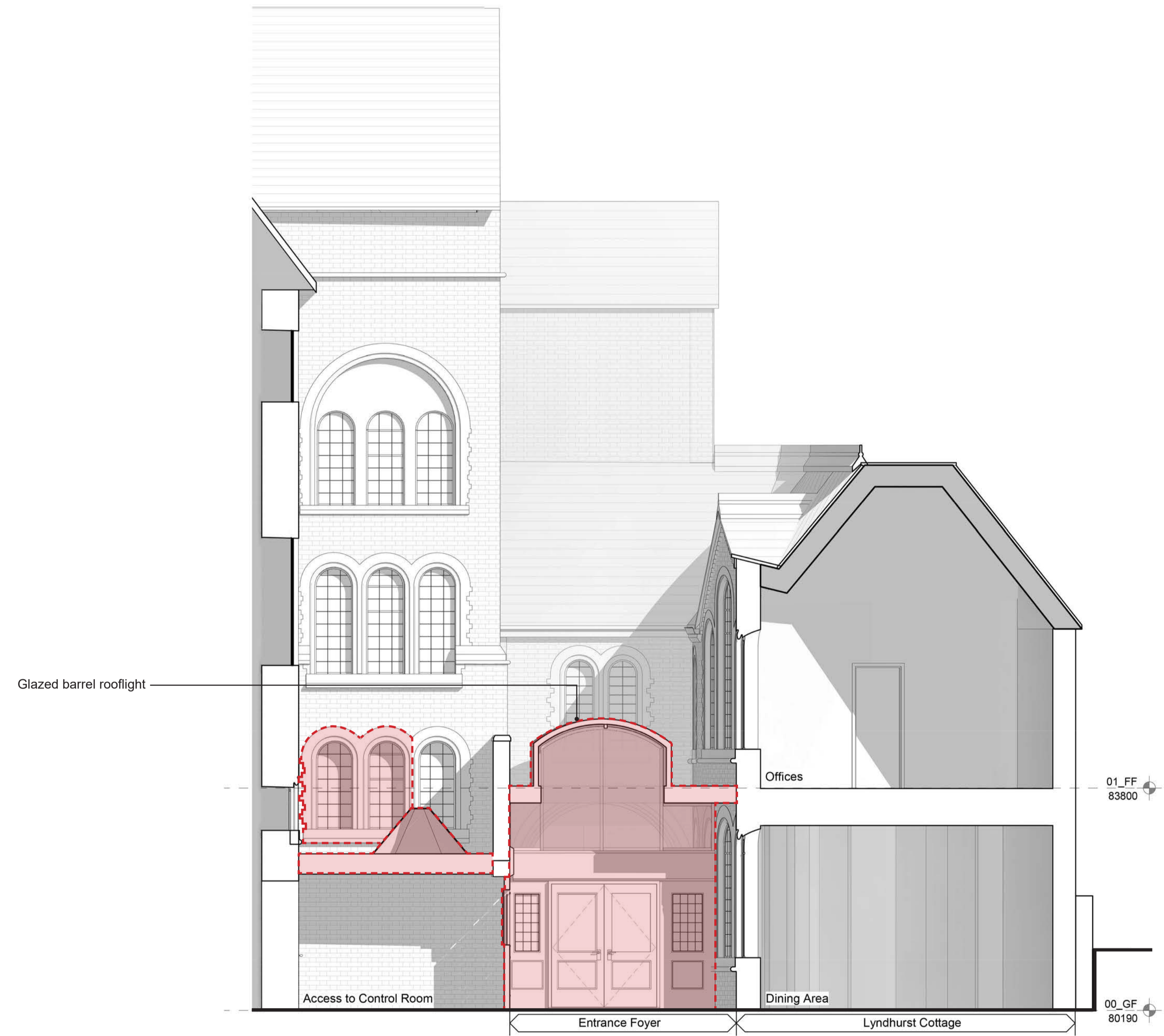
2 Existing Section B-B P005 Scale - 1 : 50
