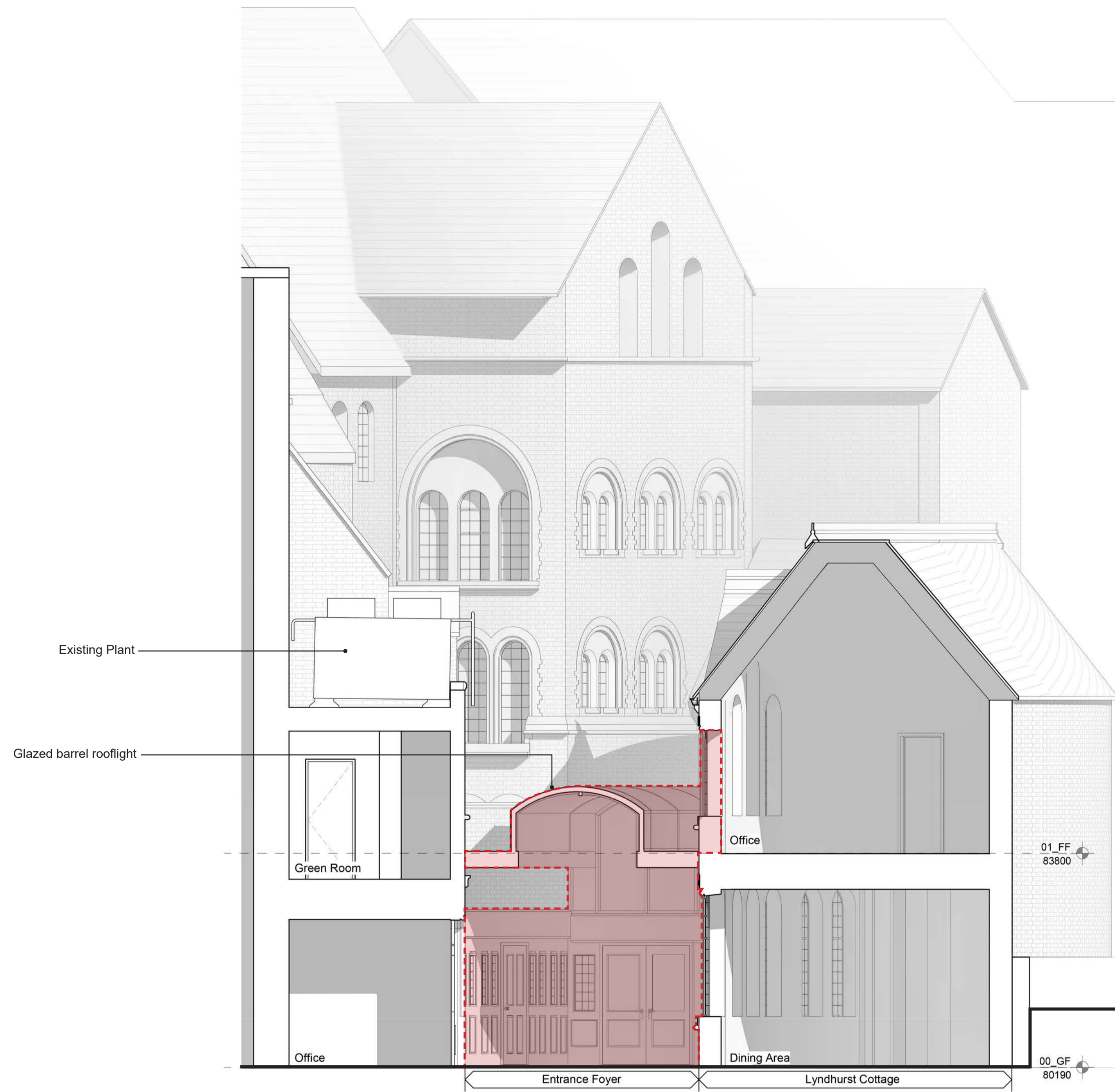
1 Existing Section A-A P005 Scale - 1 : 50
