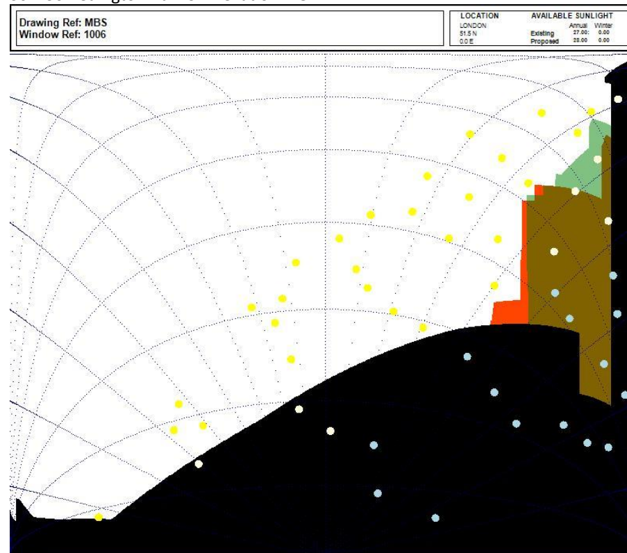
S6 – 30 Redington Rd – SE Elevation – GF
