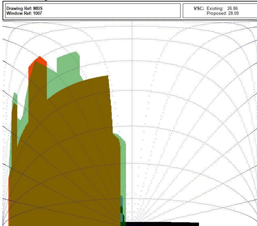
S7 – 30 Redington Rd – SE Elevation – 1F
