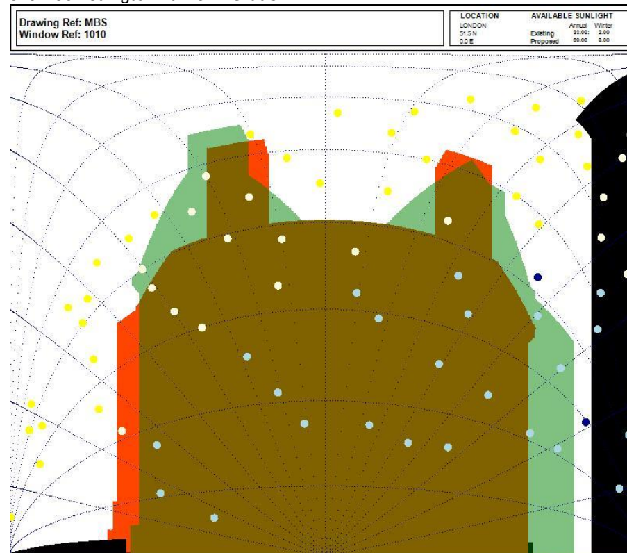
S10 – 30 Redington Rd – SE Elevation – 1F
