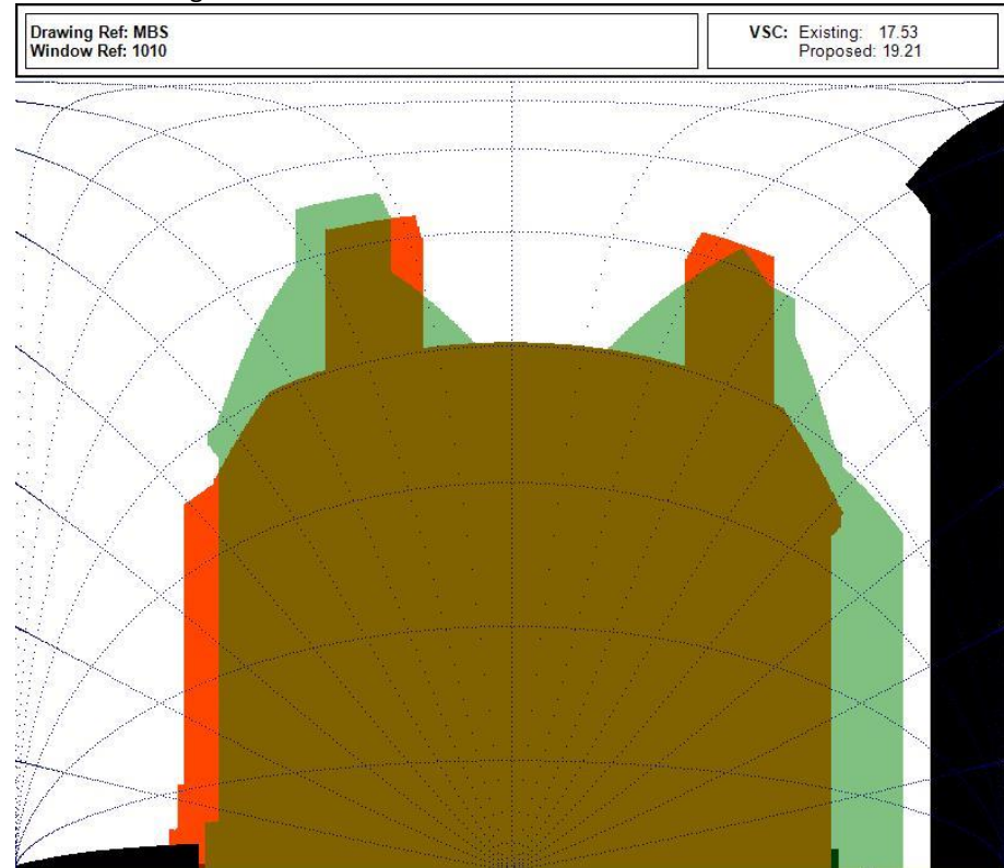
S10 – 30 Redington Rd – SE Elevation – 1F
