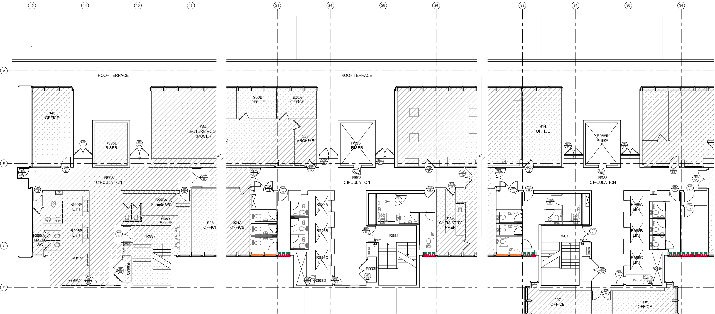
2 LEVEL 9 - CORE C PROPOSED PLAN 1:100
