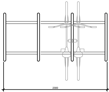
BICYCLE PLAN - 1:50
