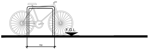
BICYCLE SHELTER - SIDE ELEVATION 1:50
