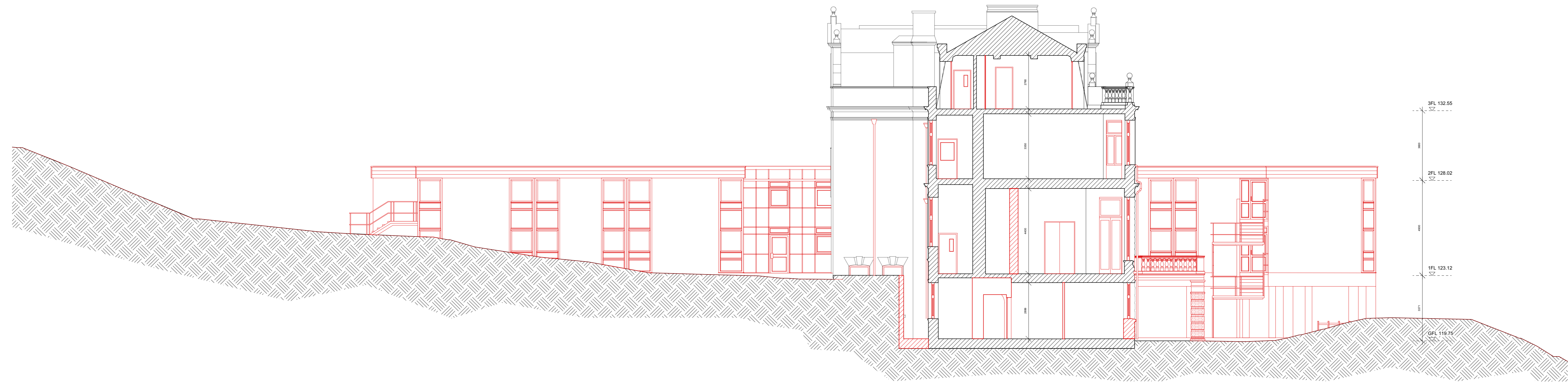
1 EXISTING AND REMOVAL SECTION F-F PL-16 Scale: 1:100
