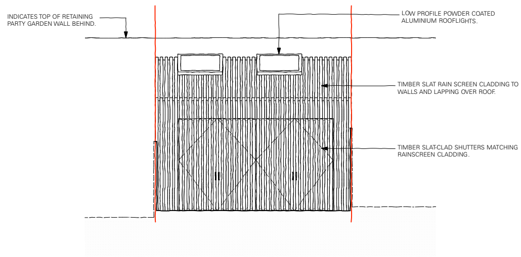
2 ELEVATION: PROPOSED, FRONT - SHUTTERS DRAWN. 1:100 @ A3
