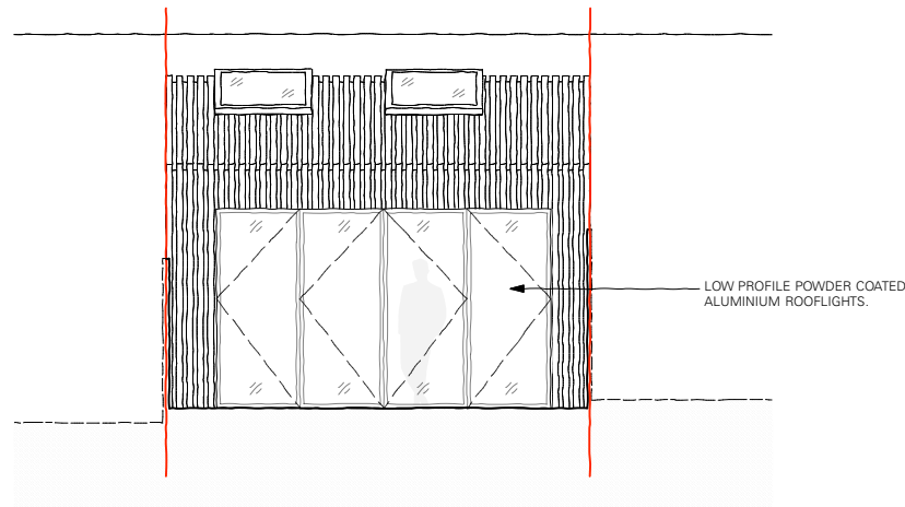
4 ELEVATION: PROPOSED, FRONT. 1:100 @ A3
