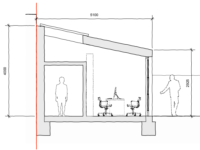
1 SECTION: PROPOSED. 1:100 @ A3
