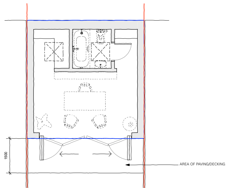
7 PLAN: PROPOSED, GROUND FLOOR. 1:100 @ A3
