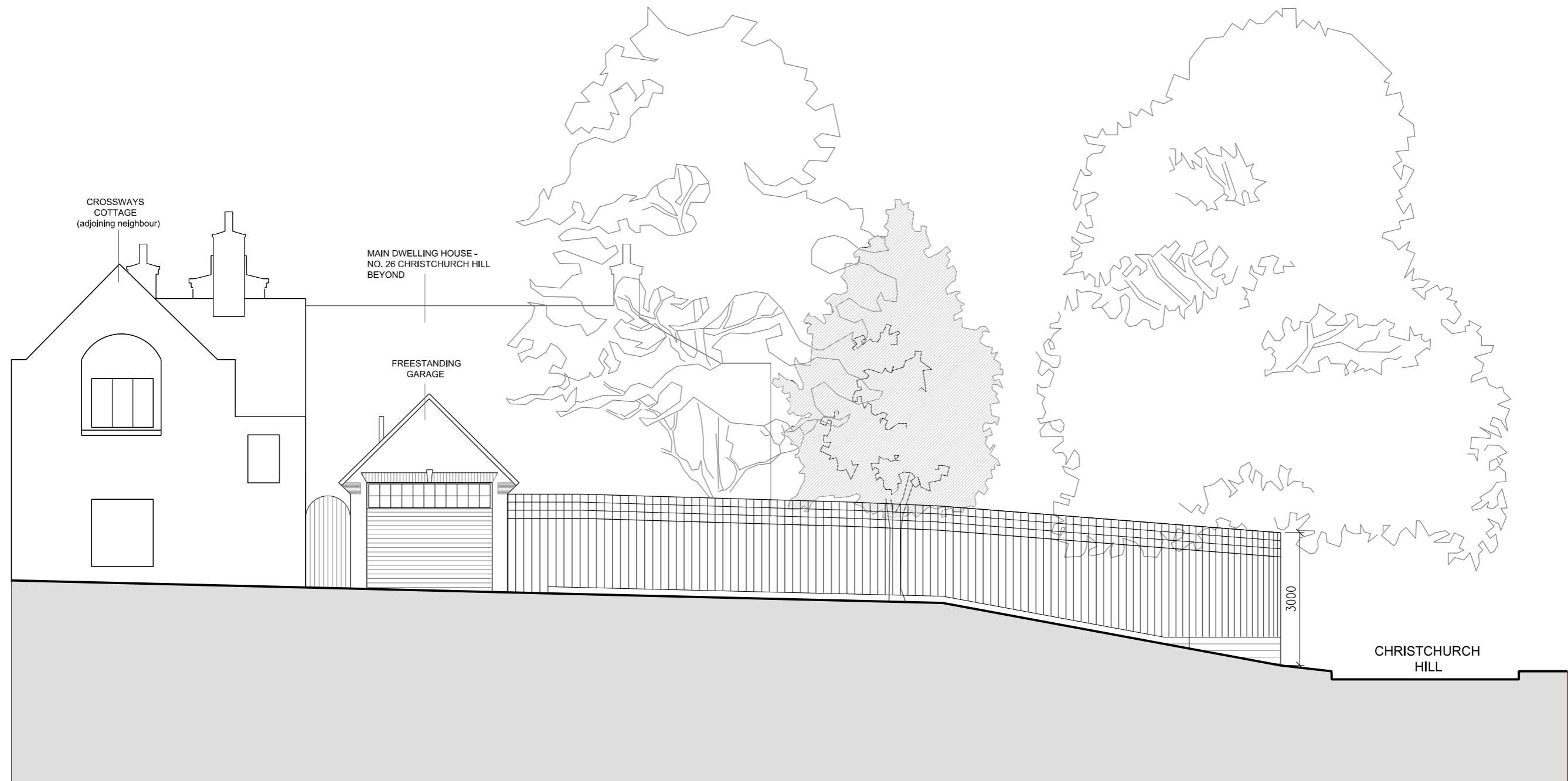
1 EXISTING SIDE BOUNDARY FENCE - TIMBER CLOSEBOARDS FRONTING WELL ROAD
