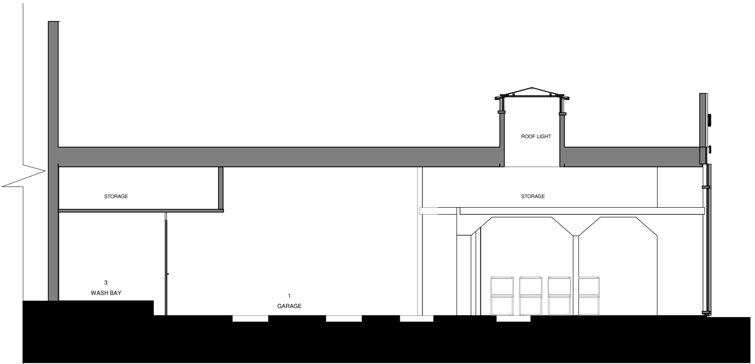
1 SECTION 1-1 1:50
