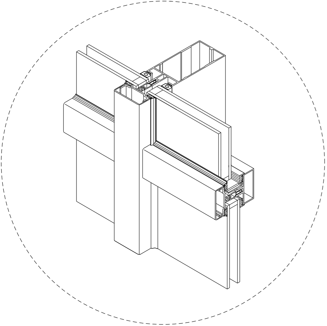
Proposed Aluminium Transom and Mullion framework
