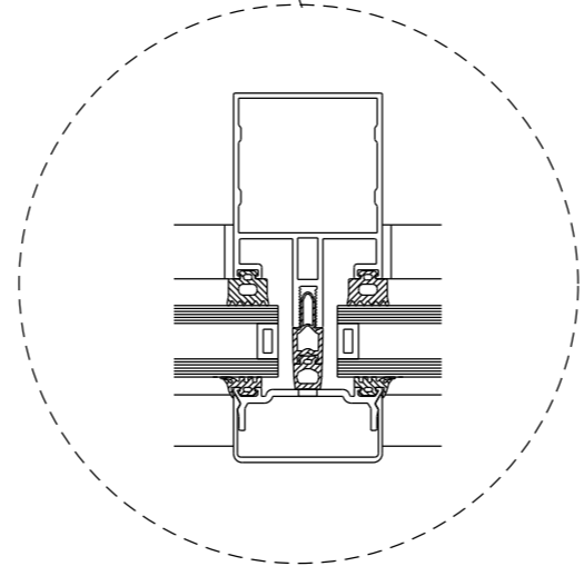
Proposed Aluminium Mullion framework
