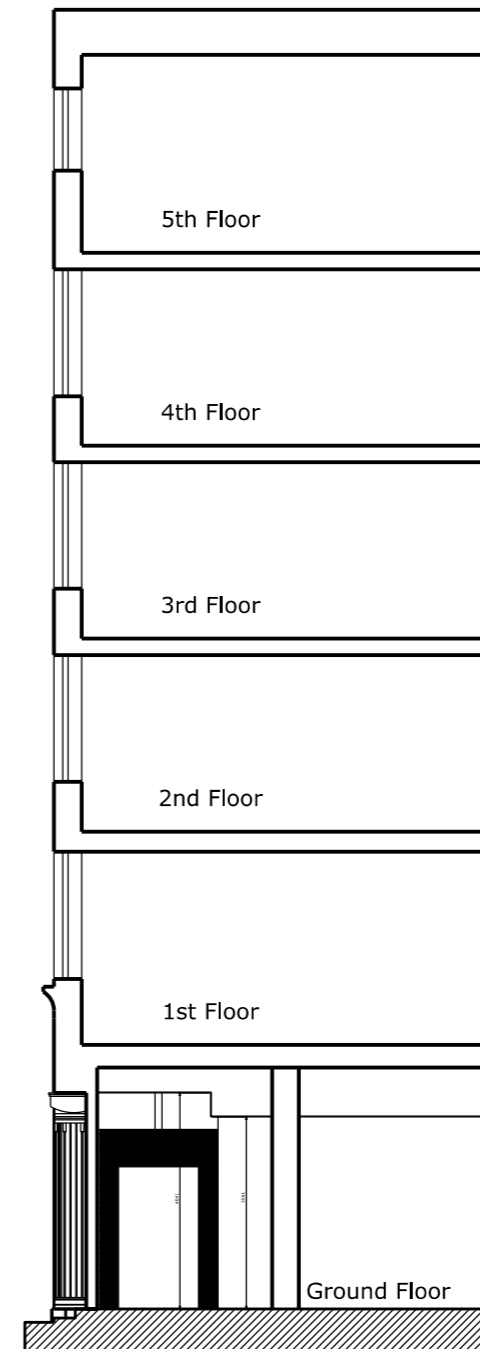
Existing Section thru Front
