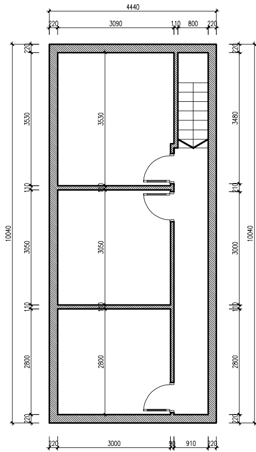
EXISTING BASEMENT SCALE 1/100
