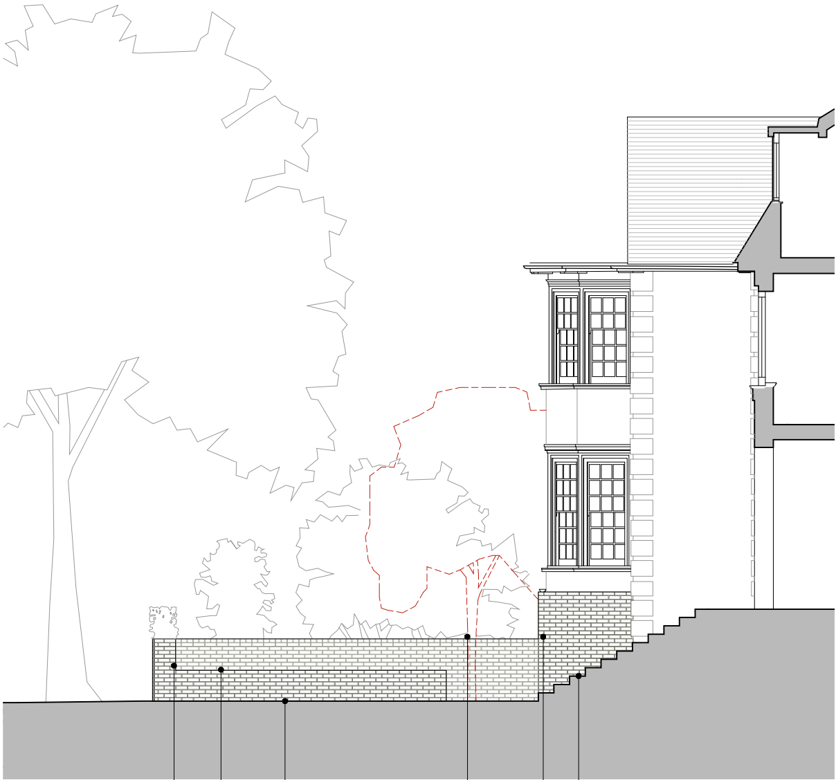
P206.02 PROPOSED SECTION E
