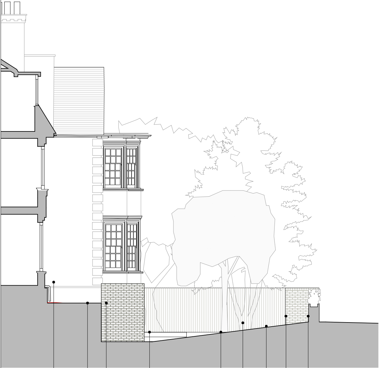
P206.01 PROPOSED SECTION D
