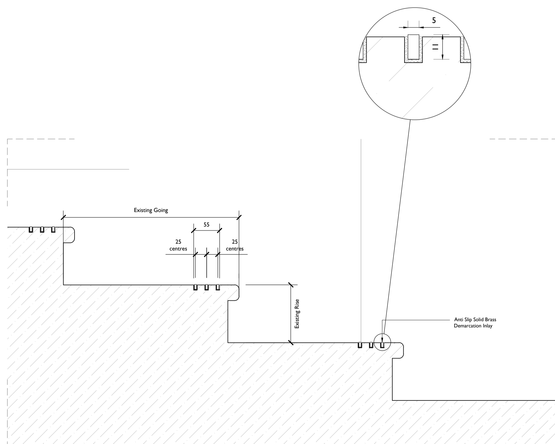
2 G0.01 Proposed Stair Nosing Detail 98031 1:5 @ A1
