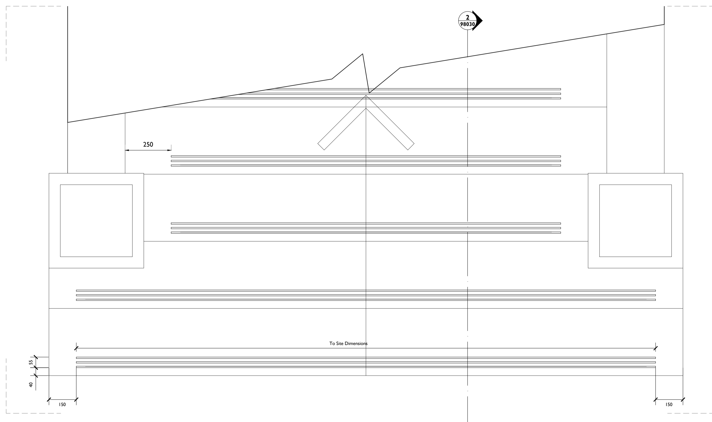
3 Proposed Grand Staircase 98031 1:10 @ A1
