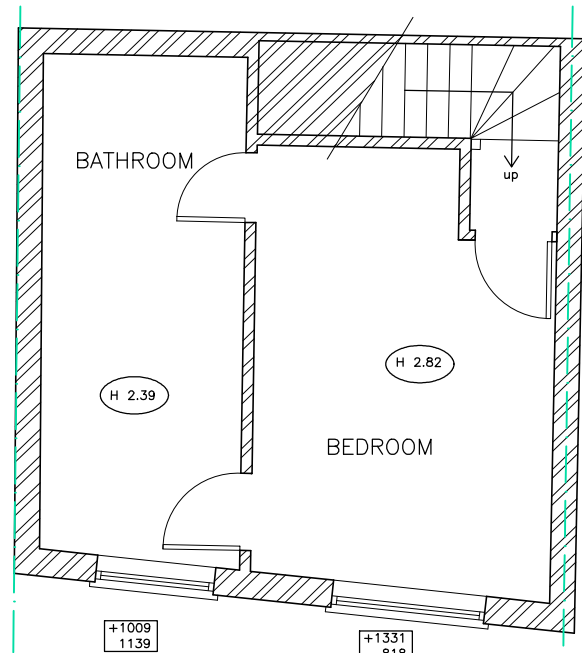
FIRST FLOOR SCALE 1:75
