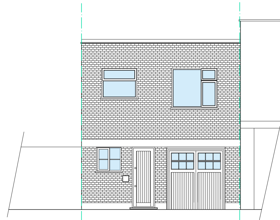
FRONT ELEVATION SCALE 1:75
