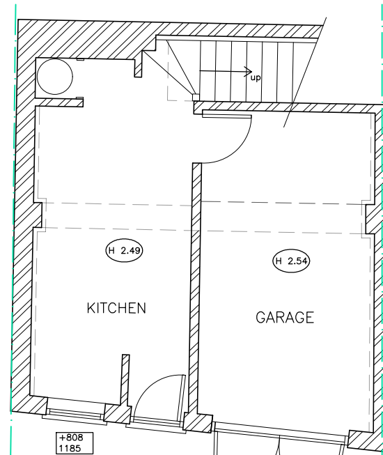
GROUND FLOOR SCALE 1:75
