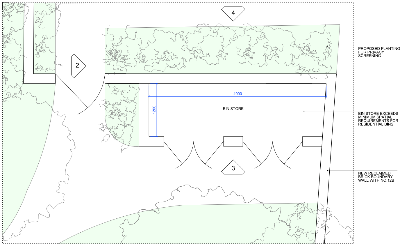
1 1:25 / 1:50 PROPOSED BIN STORE, PLAN
