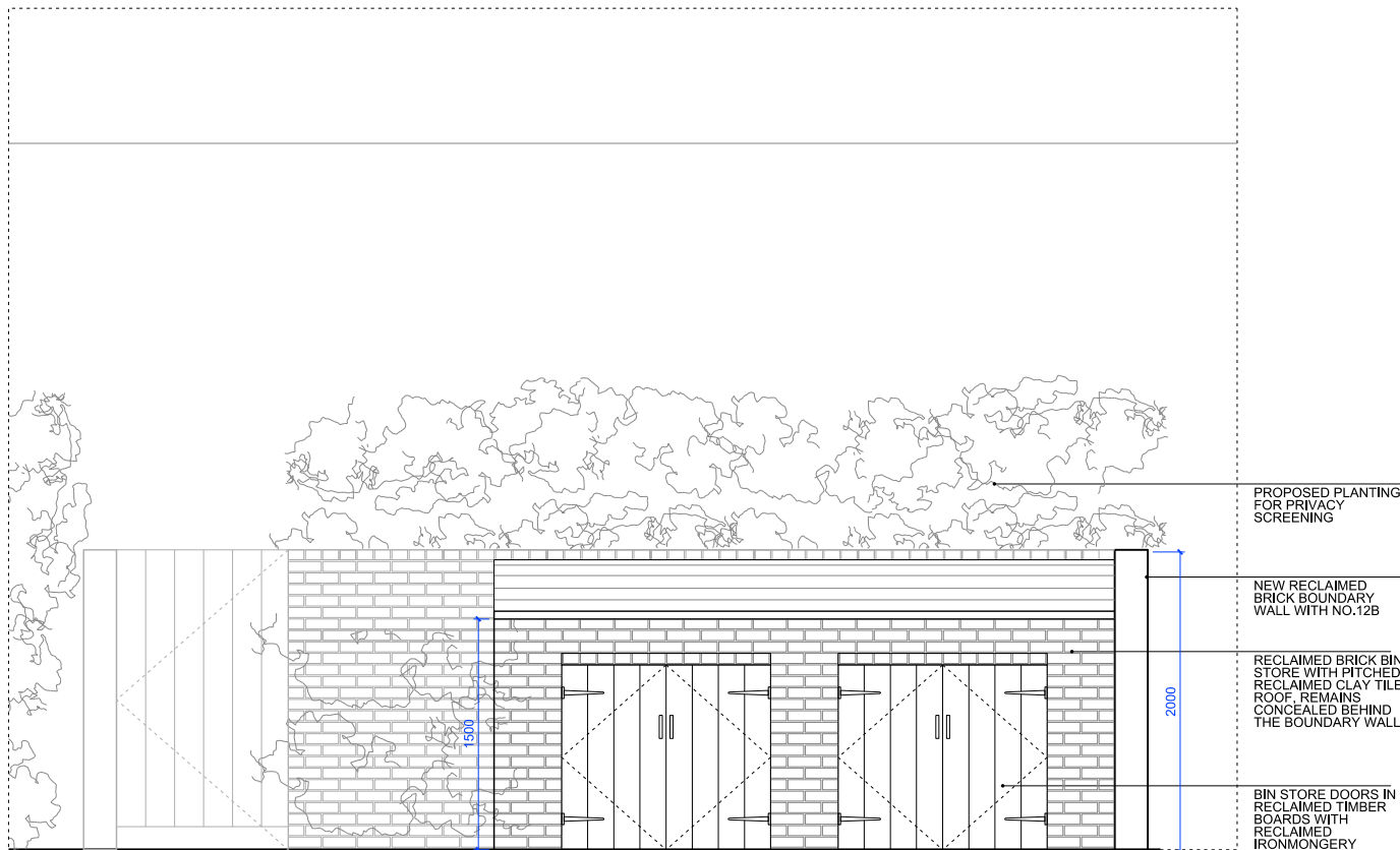
3 1:25 / 1:50 PROPOSED BIN STORE, INTERNAL FACE ELEVATION
