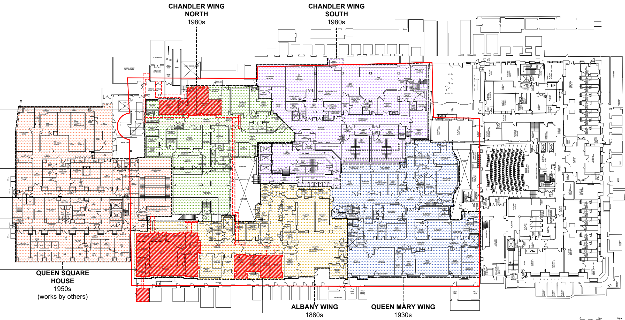
Basement Plan
