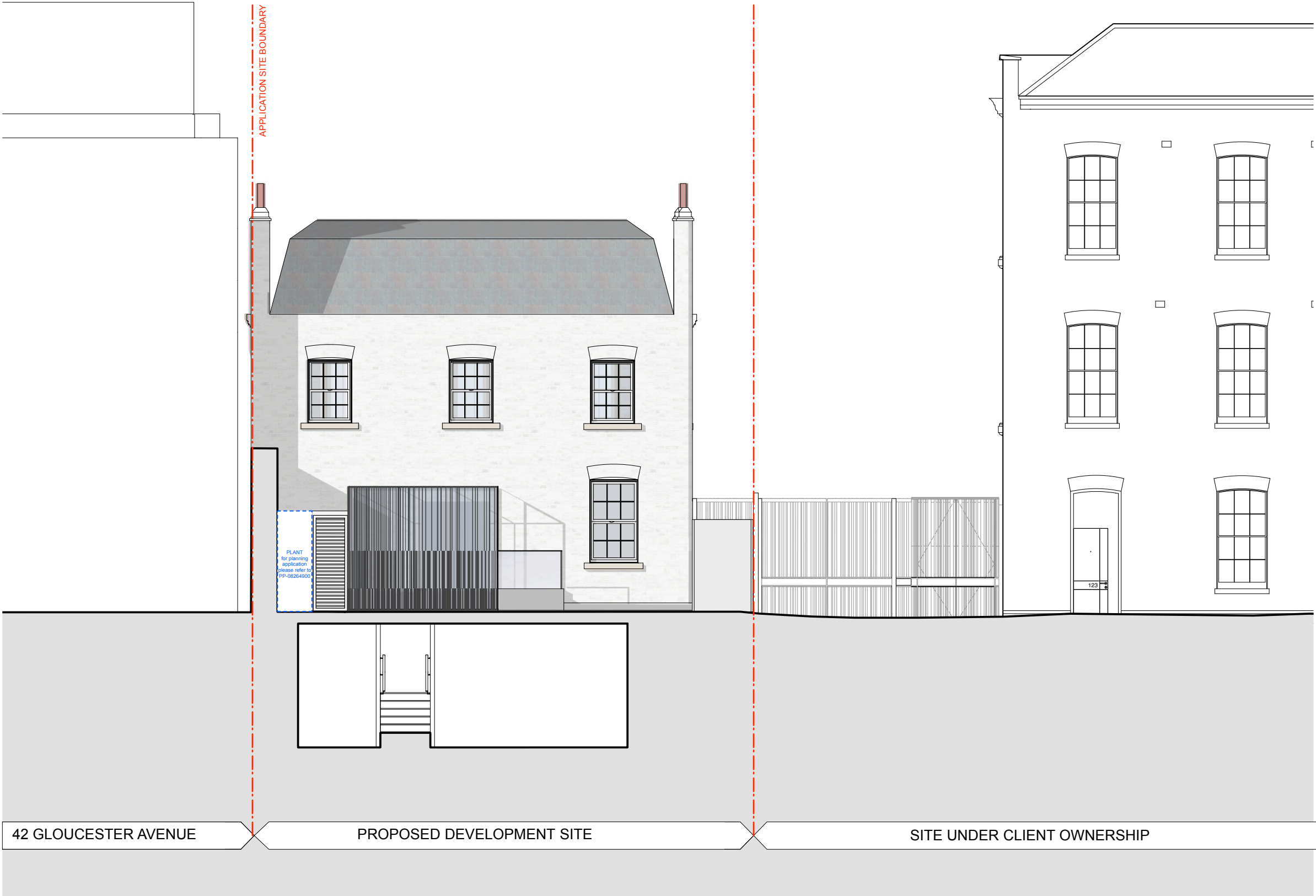
01 Proposed Elevation Gloucester Avenue 1:100 @ A1, 1:200 @ A3
