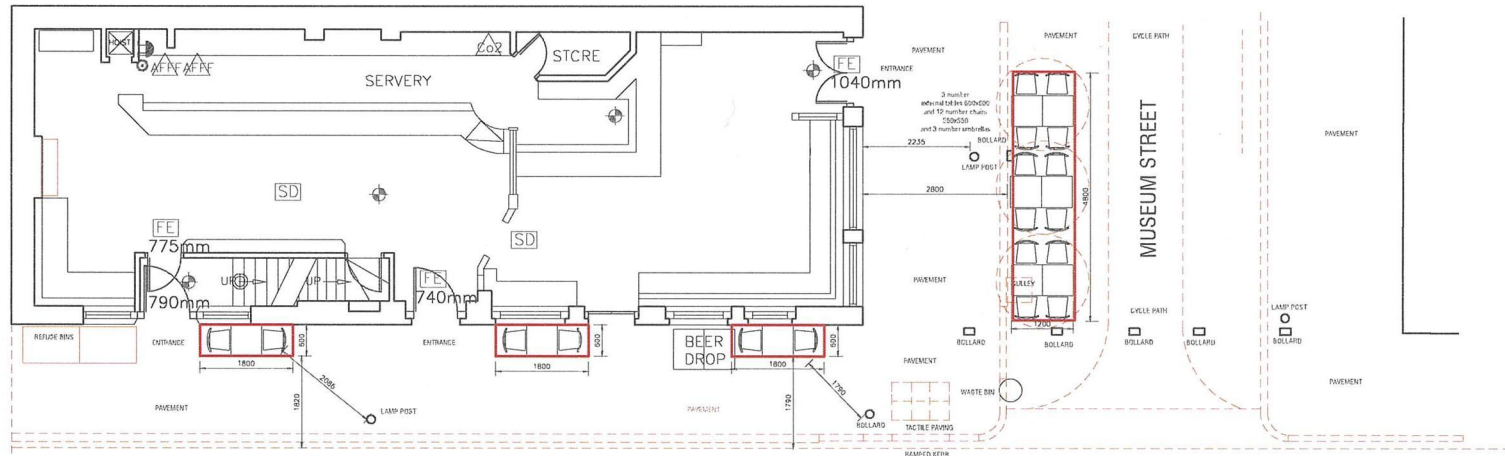
EXISTING GROUND FLOOR LAYOUT LITTLE RUSSELL STREET
